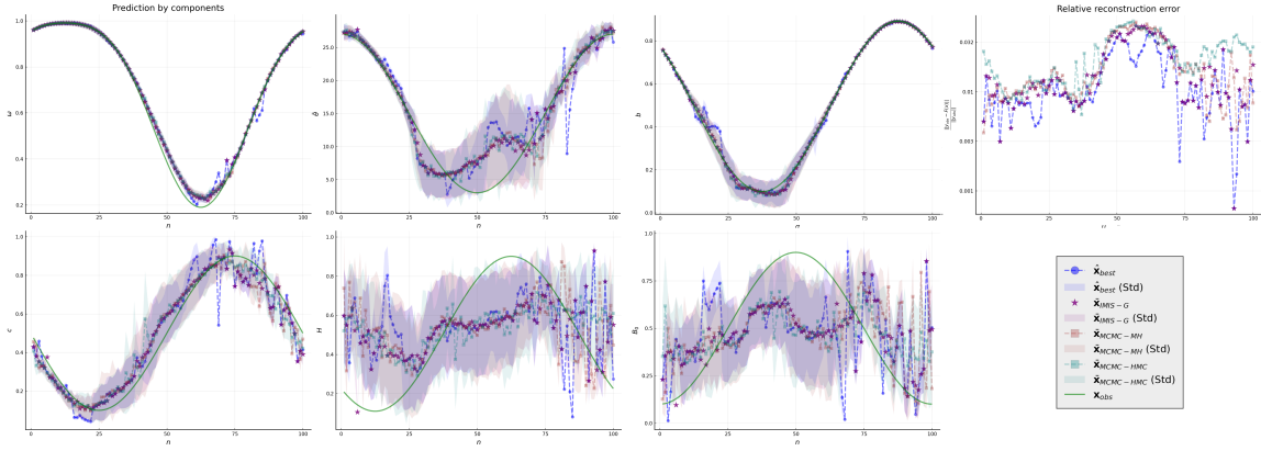
Fig. 4 Inversion of high dimensional synthetic data from the 6 parameter Hapke model. A GLLiM model is learned from training data with K = 100 . The importance sampling mean \bar{\mathbf{x}}_{IMIS-G} (star, purple) and the MCMC means (dash, brown and teal) are compared. The values to be recovered \mathbf{x}_{obs} are in green. Relative reconstruction errors are shown with a logarithmic scale in the top right plot.
