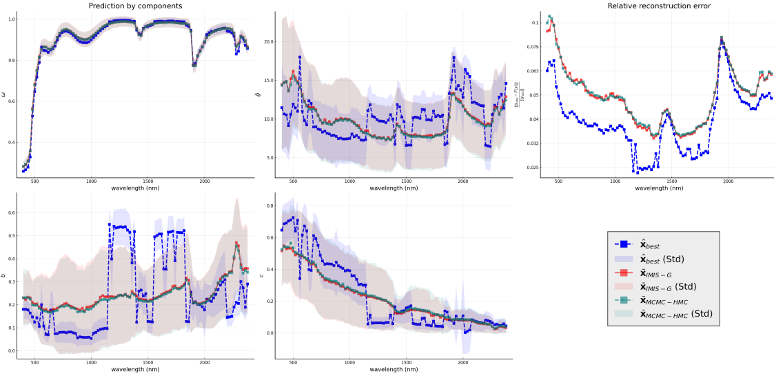
Fig. 5 Inversion of Nontronite laboratory observations. A GLLiM model is learned from training data with K = 100 . The GLLiM mean prediction refined with importance sampling \tilde{\mathbf{x}}_{MIS-G} (red), the reconstruction best prediction \hat{\mathbf{x}}_{best} (blue) and the MCMC prediction (teal) are compared. Standard deviations are also shown. Relative reconstruction errors are shown with a logarithmic scale in the top right plot.
