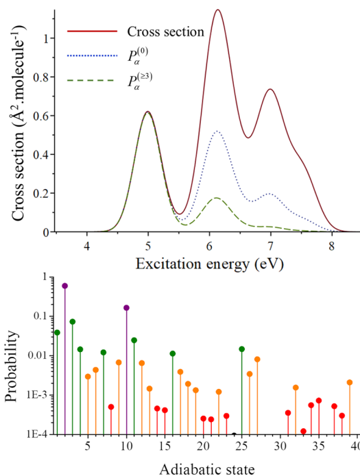
Figure 3. Top: absorption cross-section and excitation probabilities as a function of the excitation energy (eq 17) for adenine. The probability curves were normalized by the maximum of the first cross-section band. Bottom: Excitation probability ( P_\alpha^{(3)} ) of each adiabatic state S_\alpha . Numerical values for energies, oscillator strengths, and probabilities are given in Table SI-1. The bar colors indicate the oscillator strength intensity, increasing from red to violet.
