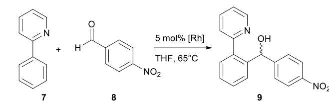
Scheme 4 Reaction of 2-phenylpyridine with 4-nitrobenzaldehyde.
