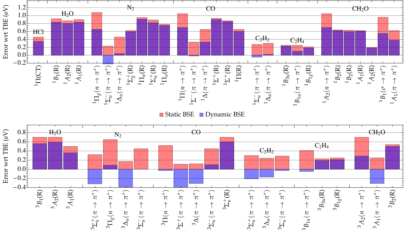
FIG. 1. Error (in eV) with respect to the TBEs of Refs. 29–31 for singlet (top) and triplet (bottom) excitation energies of various molecules obtained with the aug-cc-pVTZ basis set computed within the static (red) and dynamic (blue) BSE formalism. CT and R stand for charge transfer and Rydberg state, respectively. See Tables II and III for raw data.
