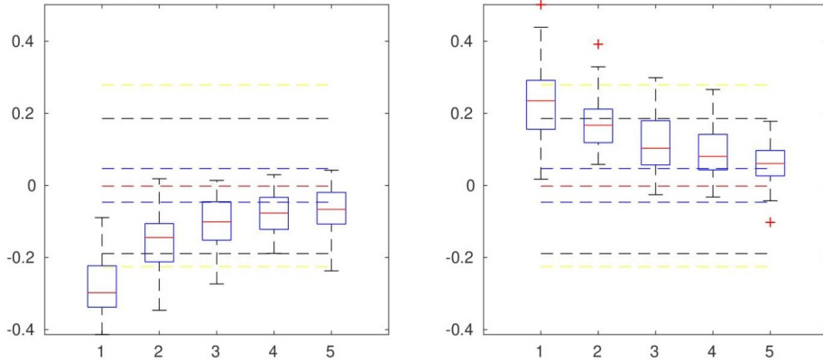
Figure 8: For r = 0.5 and d = 3 , left: box-plots of E_i^{CH} , right: box-plots of E_i^{DW} , for n = 200, 400, 600, 1000 and 2000 .
