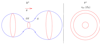
Figure 5: (c) 3D peanut
