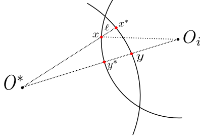
Figure 10: x \in \partial C_{\alpha'}(\mathbb{X}_n) , x^* = \pi_{\partial S}(x) , O_i = x + \alpha' \hat{\eta}_{x,i} and O^* = x^* - \alpha \eta_{x^*}
