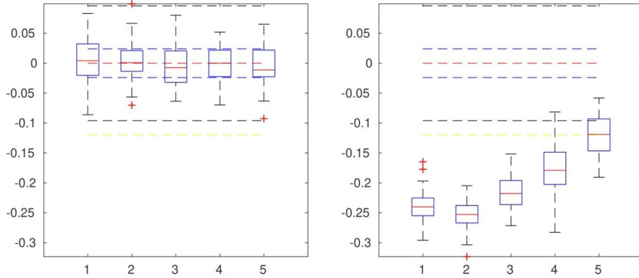
Figure 7: For r = 0.5 and d = 2 , left: box-plots of E_i^{CH} , right: box-plots of E_i^{DW} , for n = 200, 400, 600, 1000 and 2000 .
