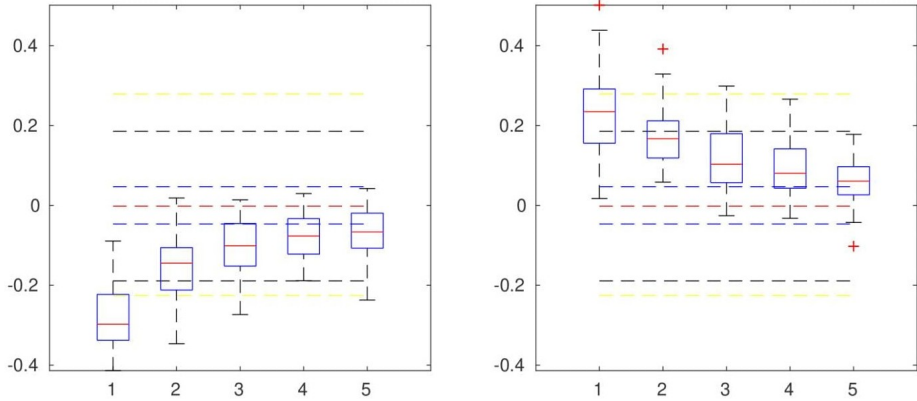
Figure 8: For r = 0.5 and d = 3 , left: box-plots of E_i^{CH} , right: box-plots of E_i^{DW} , for n = 200, 400, 600, 1000 and 2000 .
