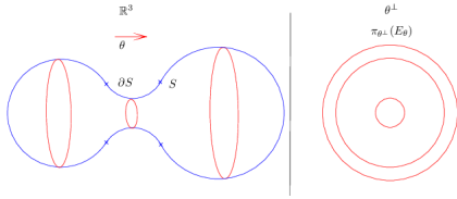
Figure 5: (c) 3D peanut
