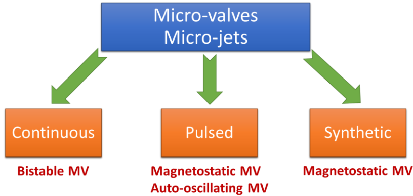
Figure 1: The 3 types of MMMS IEMN/LEMAC-LICS Microvalves dedicated to microjets for active aerodynamic flow control
