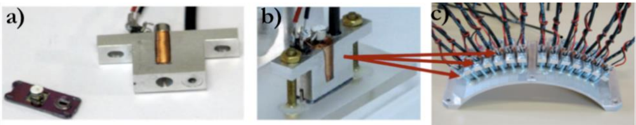
Figure 6: Magneto static pulsed micro valves with packaging allowing easy individual mounting on no conformal Geometries for separation control. Micro jet velocities >100\text{m/s} , frequency range [50 Hz, 700 Hz].
