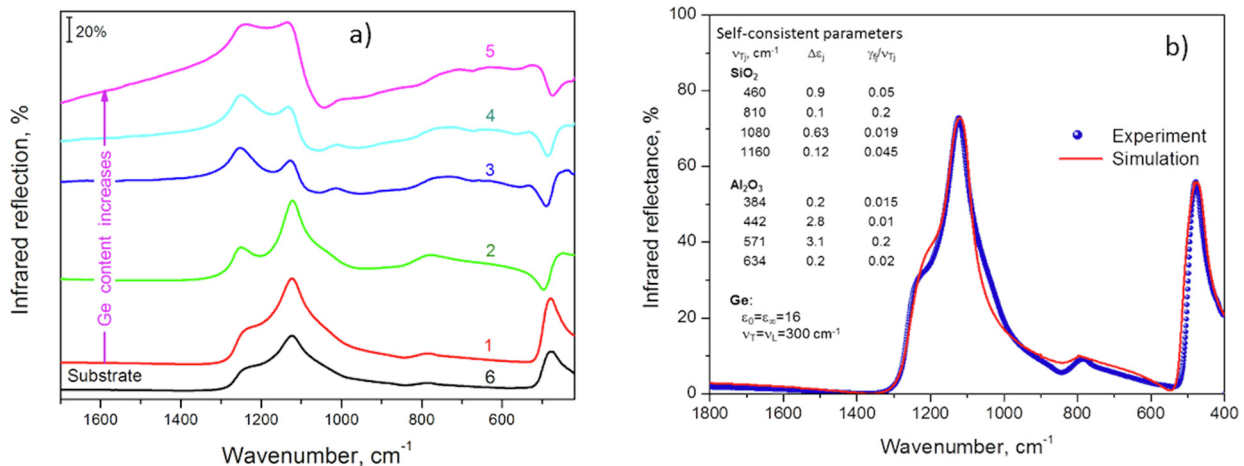
Fig. 2. a) Specular IRR spectra for the films with [Ge] = 20(1), 24(2), 30(3), 36(4), 42(5). Curve 6 corresponds to the quartz substrate; b) simulation of specular IRR spectrum for the film with [Ge] = 20%.
