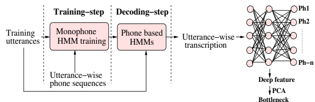
Figure 1: Phone-BN feature extraction system.
