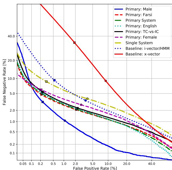
Figure 2: DET plots of the UIAI systems along with baselines.
