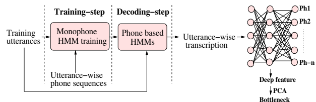
Figure 1: Phone-BN feature extraction system.
