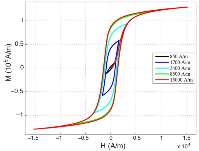
Fig. 2. Experimental results: magnetic hysteresis at increasing magnetic field levels without applied stress – M = f(H, \sigma = 0 \text{ MPa}) .
