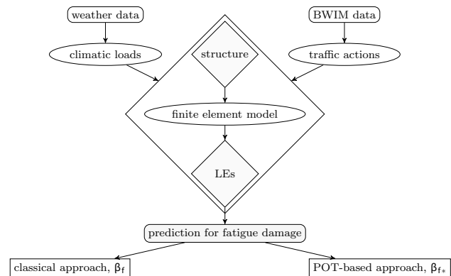
Fig. 1 General methodology, from monitoring to reliability
