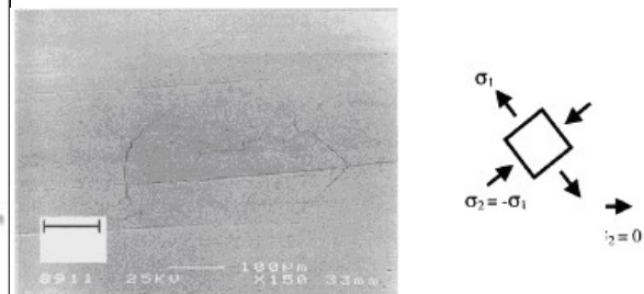
Figure 4: Fatigue cracks during torsion of C45 low carbon steel
