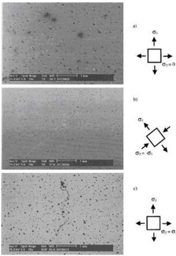
Figure 3: Fatigue cracks during a) axial tension, b) torsion, and c) equi-biaxial tension loading for FCD700
