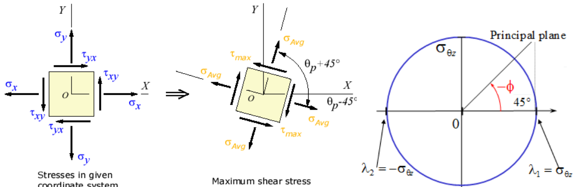
Figure 16: Transformation of the Maximum Shear Stress Directions and Mohr's Circle for Torsional Loading Mohre circle
