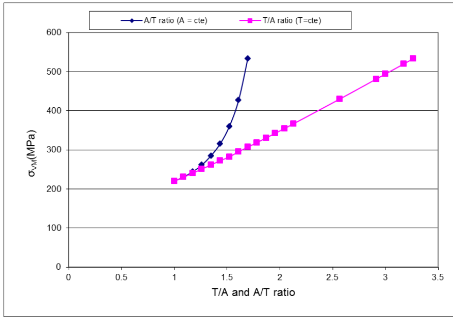
Figure 13: Effect of Stress Ratio on Maximum Von Mises Stress
