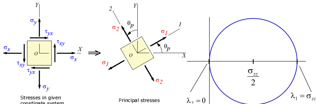
Figure 15: Transformation of the Maximum Principal Stress Directions and Mohr's Circle for Axial Loading Mohre circle
