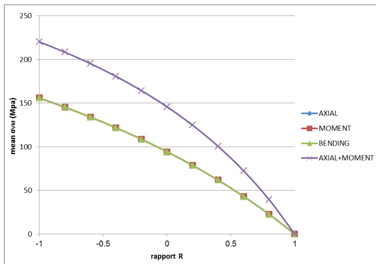
Figure 11: Effect of R on Mean Von Mises Stress
