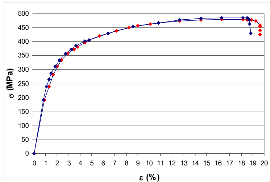
Figure 6: Tensile Test Curves
