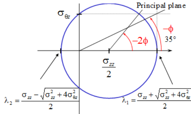
Figure 17: Mohr's Circle for Axial-Torsional Loading Mohre circle
