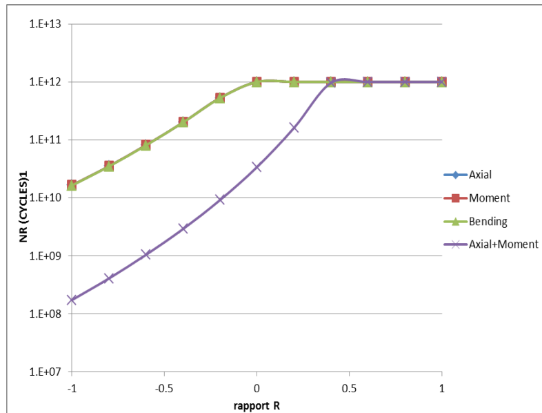
Figure 12: Effect of R on Mean Fatigue Life
