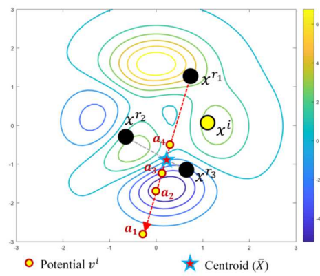
Fig. 4. NM-based-rand/3 mutation strategy for the DE algorithm
