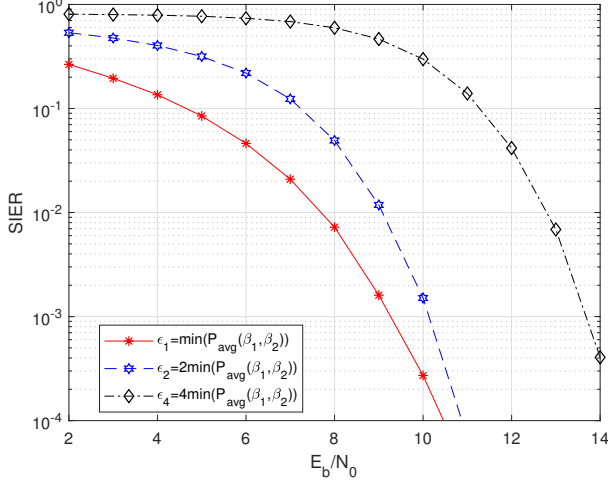
Fig. 3. SIER comparison at different thresholds for the 64-QAM over the Rayleigh fading channel without any erasure
