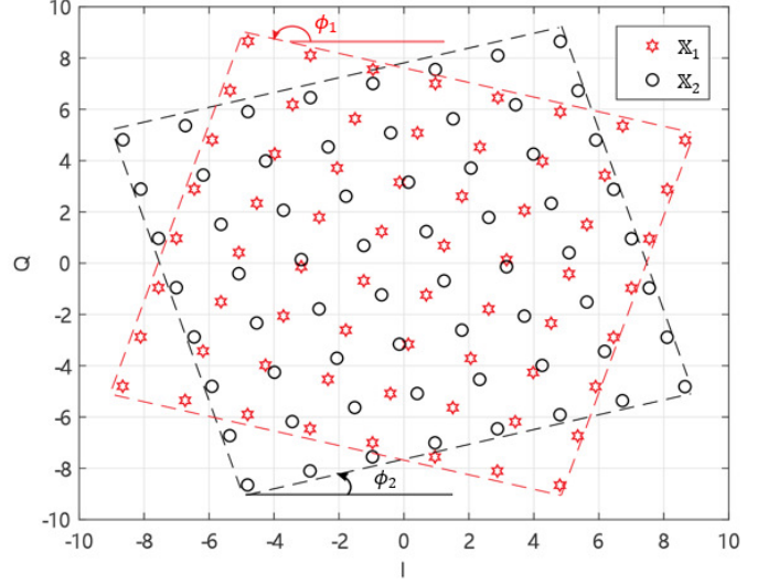
Fig. 1. Rotated constellations \mathbb{X}_1 and \mathbb{X}_2 for the 64-QAM signal
