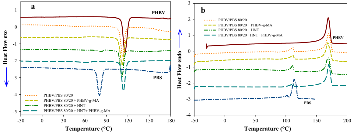
Fig. 10. DSC thermograms of PHBV/PBS 80/20 binary blend and PHBV/PBS/HNT nanocomposites with and without PHBV-g-MA compatibilization: (a) cooling scan and (b) heating scan.
