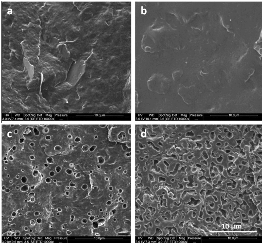
Fig. 2. SEM micrographs of cryo-fractured surfaces of neat PHBV (a), neat PBS (b) and PHBV/PBS blends after selective etching of PBS with chloroform, 80/20 w/w (c), 50/50 w/w (d). Holes correspond to the PBS nodules.
