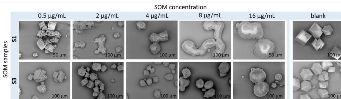
Figure 8: SEM images of the in vitro \text{CaCO}_3 crystallization assay in the presence of Spondylus ASMs (fractions S1 and S3) tested at different concentrations: the effect of ASMs was tested at increasing concentrations of 0.5, 2, 4, 8 and 16 \mu\text{g}\cdot\text{mL}^{-1} .
