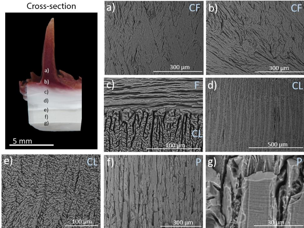
Figure 2: SEM micrographs of the microstructures observed along a polished transversal section of Spondylus gaederopus shell (upper valve): a) calcitic crossed-foliated (CF) structure of the spine; b) irregular calcitic CF microstructure observed at the point of spine formation; c) transition between the calcitic foliated (F) and the aragonitic crossed-lamellar (CL) structures; d) aragonitic crossed-lamellar (CL) structure in the upper part of the shell; e) aragonitic crossed-lamellar (CL) structure in the lower part of the section; f,g) aragonitic prismatic (P) layer in the bottom part of the shell and myostracum. Structural abbreviations: F - calcitic foliated; P - aragonitic prismatic; CL - aragonitic crossed-lamellar, CF - calcitic crossed-foliated.
