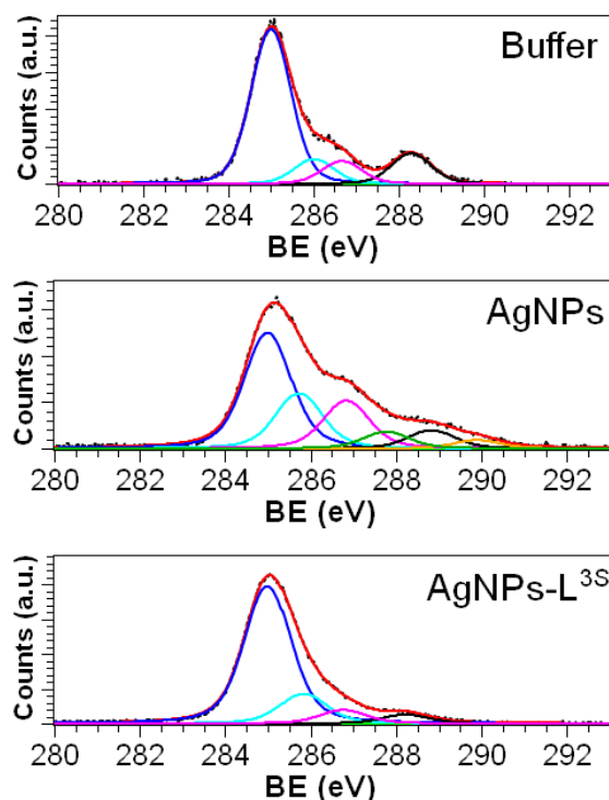
Figure 5. SR-XPS spectra of C 1s core level for the 2 mM Na-citrate buffer solution, uncoated AgNPs, and the L^{3S} -AgNPs solution. Best-fitting curves are reported in red over the corresponding experimental spectrum (black dots). Individual Voigt components contributing to the final fit are reported on each graph (blue, cyan, magenta, green, black, orange solid curves). Photon energy 596 eV.
