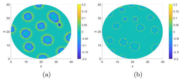
Figure 11: Difference between the solutions u(\mathbf{x}, 200) - w(\mathbf{x}, 230) when (a) A = B = 20 and (b) A = B = 70 . Here \gamma_M = 11 , r_0 = 0.05 and u_{\max} = u_0 = 0.1 .
