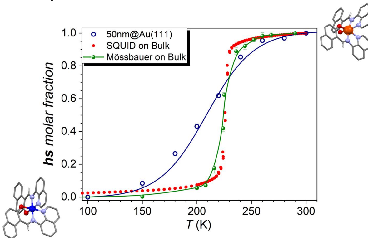
Figure 1. Comparison between bulk SQUID magnetic characterization (red dots), Mössbauer spectroscopy of [\text{}^{57}\text{Fe}(\text{qnal})_2] in bulk (green dots, the line is a guide for the eyes) and High-Spin Fe(II) thermal distribution profile obtained from XAS on a thin film (blue dots). The blue line is the best fit to a Boltzmann distribution of the XAS data giving a T_{1/2} = 210 \pm 5 \text{ K} (originally reported in reference 18); the total electron yield mode used in ref 18 to characterize the LS-HS conversion is surface sensitive thus providing information only on the topmost molecular layers and cannot be considered informative as the SMS spectroscopy respective to the entire deposit.
