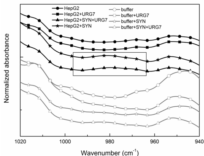
Figure 6. Raw FTIR spectra of cellular dried films and buffer preparations in the 1200–940 \text{cm}^{-1} zone.
