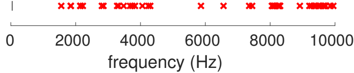
Figure 5: Eigenfrequencies of the slider up to 10 kHz, as calculated with the FE model with the bottom face fixed.
