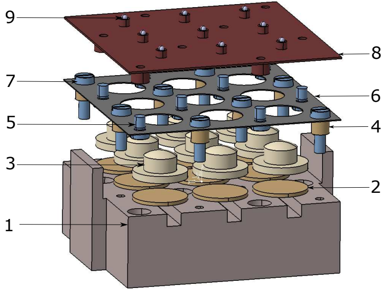
Figure 2: Exploded 3D view of the various mechanical parts constituting the instrumented slider. 1: Aluminum base. 2: Piezoelectric elements. 3: Sphere-ended aluminum fitting parts. 4: Hollow cylinder-shaped spacer. 5 & 7: M3 screws. 6: Hollow carbon steel spring plate. 8: Carbon steel top plate, featuring 8 threaded hollow cylinders on its bottom, and 9 sphere holders on its top. 9: Bearing steel sphere.
