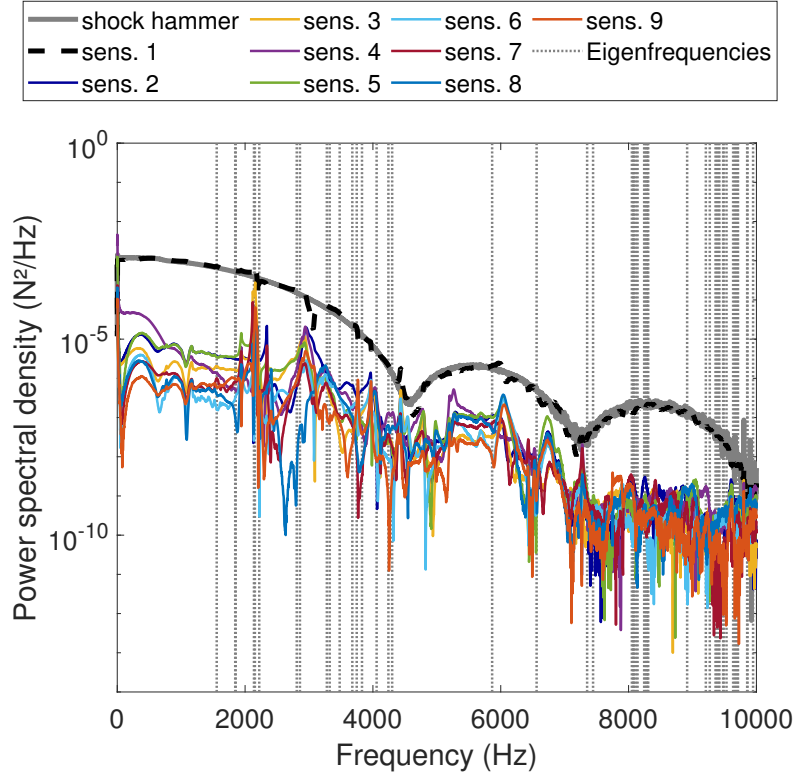
Figure 8: Average PSDs of the nine output signals from the piezoelectric sensors and from the impact hammer, over ten impacts on asperity 1, one of which is shown in Fig. 7. Dotted vertical lines: eigenfrequencies predicted by the FE modal analysis of section 2.2.
