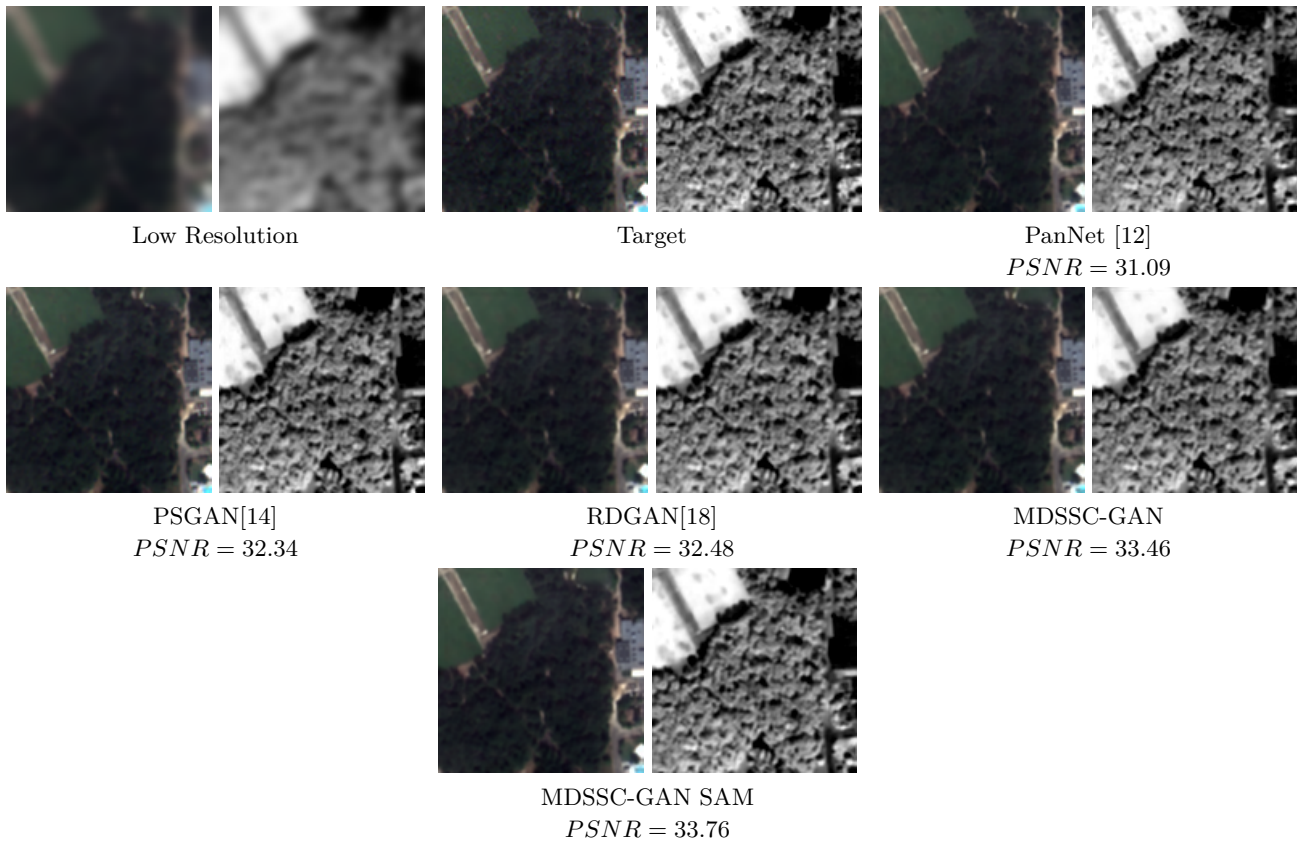
Figure 7: Visual results for state-of-the-art methods. For each method is displayed the RGB image on the left and the near infrared (NIR) band on the right. A significant improvement if the PSNR is observed with our new method MDSSC-GAN SAM.
