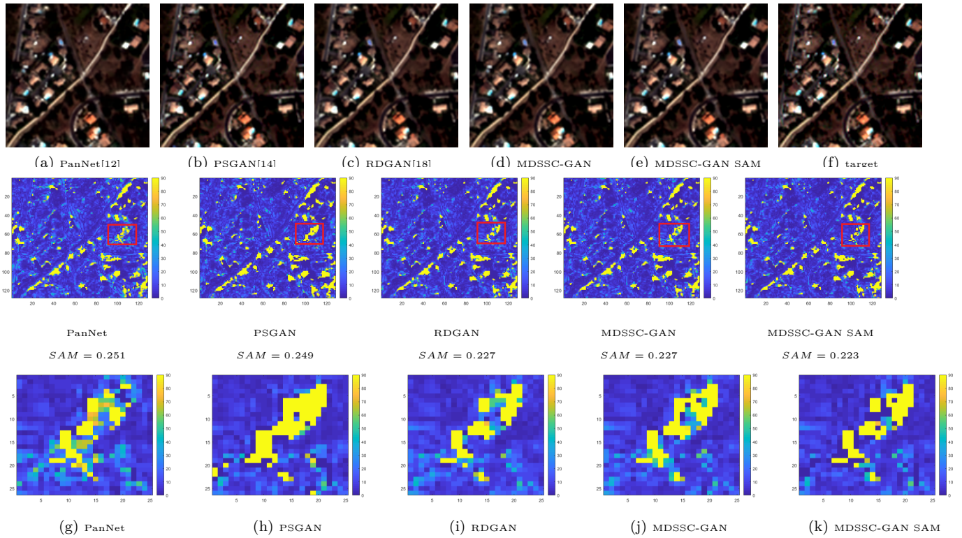
Figure 8: Visual results of state of the art methods. The first line is RGB images, the second line is the map SAM, i.e the angle of distortion between the fused image and the target at each pixel and the third line is a zoom of the map SAM. The blue indicates an angle of distortion of 0 and the yellow an angle of 90. The best result is given by the proposed MDSSC-GAN SAM method.
