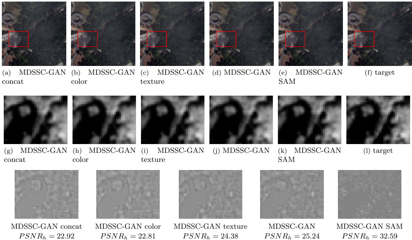
Figure 6: Visual results on vegetation areas when comparing performances of each discriminator individually with the proposed MDSSC-GAN method. MDSSC-GAN color considers only the color discriminator, MDSSC-GAN texture considers only the geometrical discriminator, MDSSC-GAN concat considers only one discriminator taking in input the concatenation of the luminance, the near infrared band and the chroma components Cb and Cr, MDSSC-GAN and MDSSC-GAN SAM are the proposed methods, the last one adding a spectral constraint to the loss function. The first line is RGB images, the second line near infrared bands and the third line differences between the high frequencies of target images with the high frequencies of fused images. We can see that the best results is given by the proposed MDSSC-GAN SAM method.
