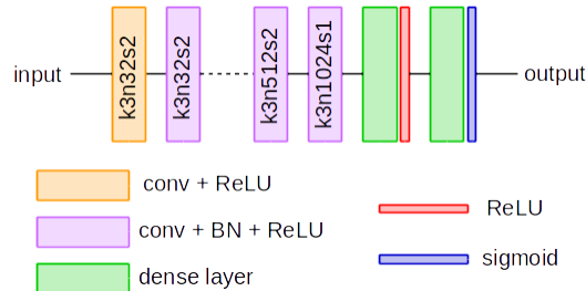
Figure 4: Architecture of each discriminator, where k is the kernel size, n the number of filters and s the stride for the convolutional layers.
