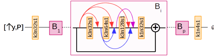
Figure 5: General architecture of the generator. The input [P, \uparrow y] is the concatenation [\cdot] of the panchromatic image P and \uparrow y the multispectral image y = (y^1, \dots, y^N) resized to the size of P , blocks B_i, i \leq p , are residual dense blocks, k is the kernel size of the convolution, n the number of filter and s the stride. Each convolutional layer is followed by a ReLU, except the last layer of the network. Arrows represent the dense connections and the + residual connection.
