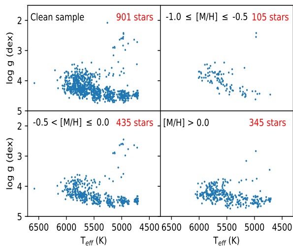
Fig. 3. HR diagram (in metallicity bins) of the selected AMBRE:HARPS stellar sample with FWHM_{CCF} \leq 8 \text{ km s}^{-1} and more than four observed spectra ( \geq 4 repeats).
