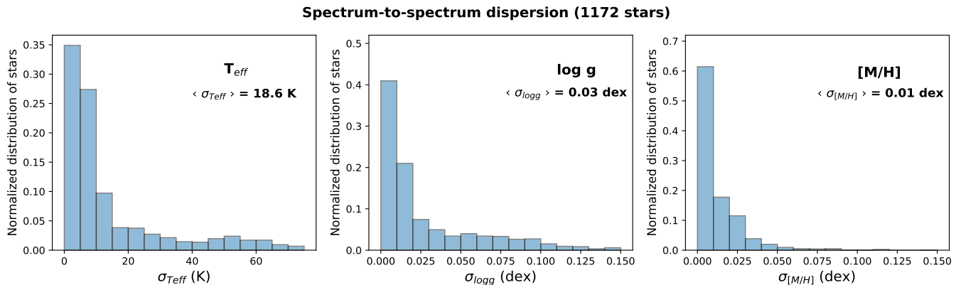
Fig. 2. Estimated dispersion of the selected stars ( \geq 4 repeats) on the effective temperature ( left ), the surface gravity ( middle ), and the global metallicity ( right ).
