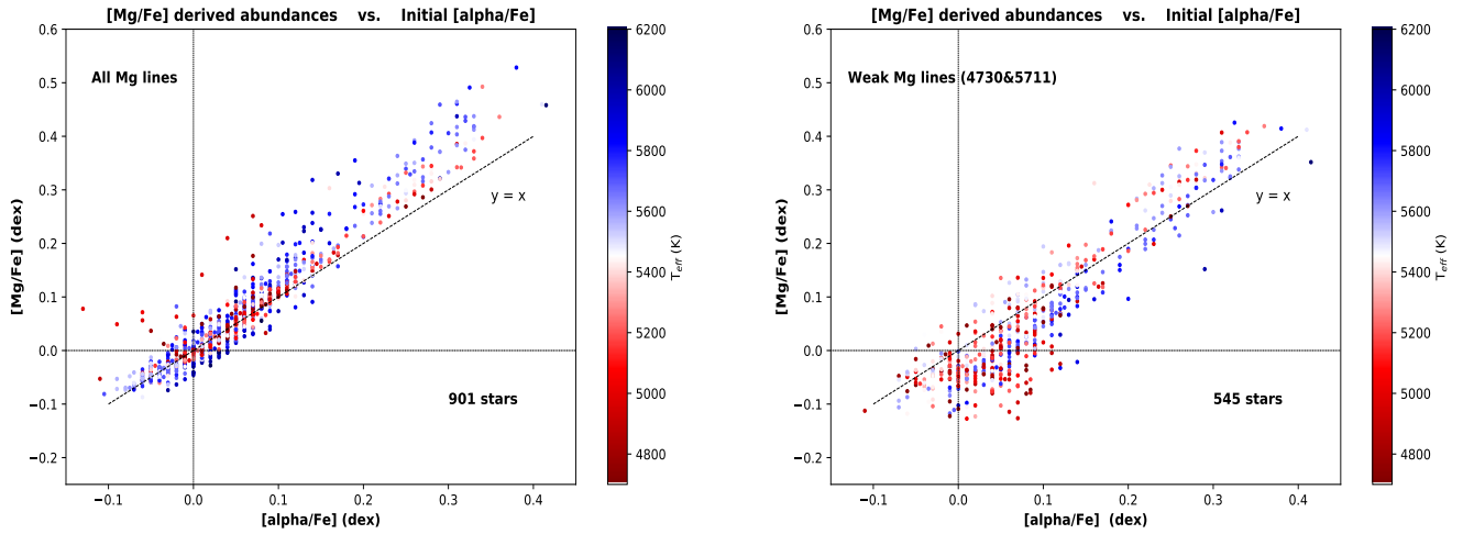
Fig. 18. Derived stellar abundance ratios [\text{Mg}/\text{Fe}] vs. initial stellar parameter [\alpha/\text{Fe}] , colour-coded by stellar effective temperature. Left: considering the abundance information from all the studied Mg I spectral lines. Right: considering only the weak non-saturated lines 4730.04 and 5711.09 Å (used in Fuhrmann et al. 2017, as the input parameter to the strong saturated lines).
