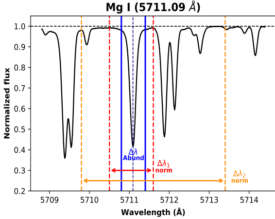
Fig. 4. Observed solar spectrum from HARPS ( R = 115\,000 , asteroid reflection) around the line 5711.09\text{ \AA} . The adopted wavelength domain where the abundance is measured is delimited by blue vertical lines ( \Delta\lambda_{\text{Abund}} \sim 0.5\text{ \AA} ). Two different local normalisation intervals of 1\text{ \AA} ( \Delta\lambda_1 ) and 4\text{ \AA} ( \Delta\lambda_2 ) are shown with red and orange dashed vertical lines, respectively.
