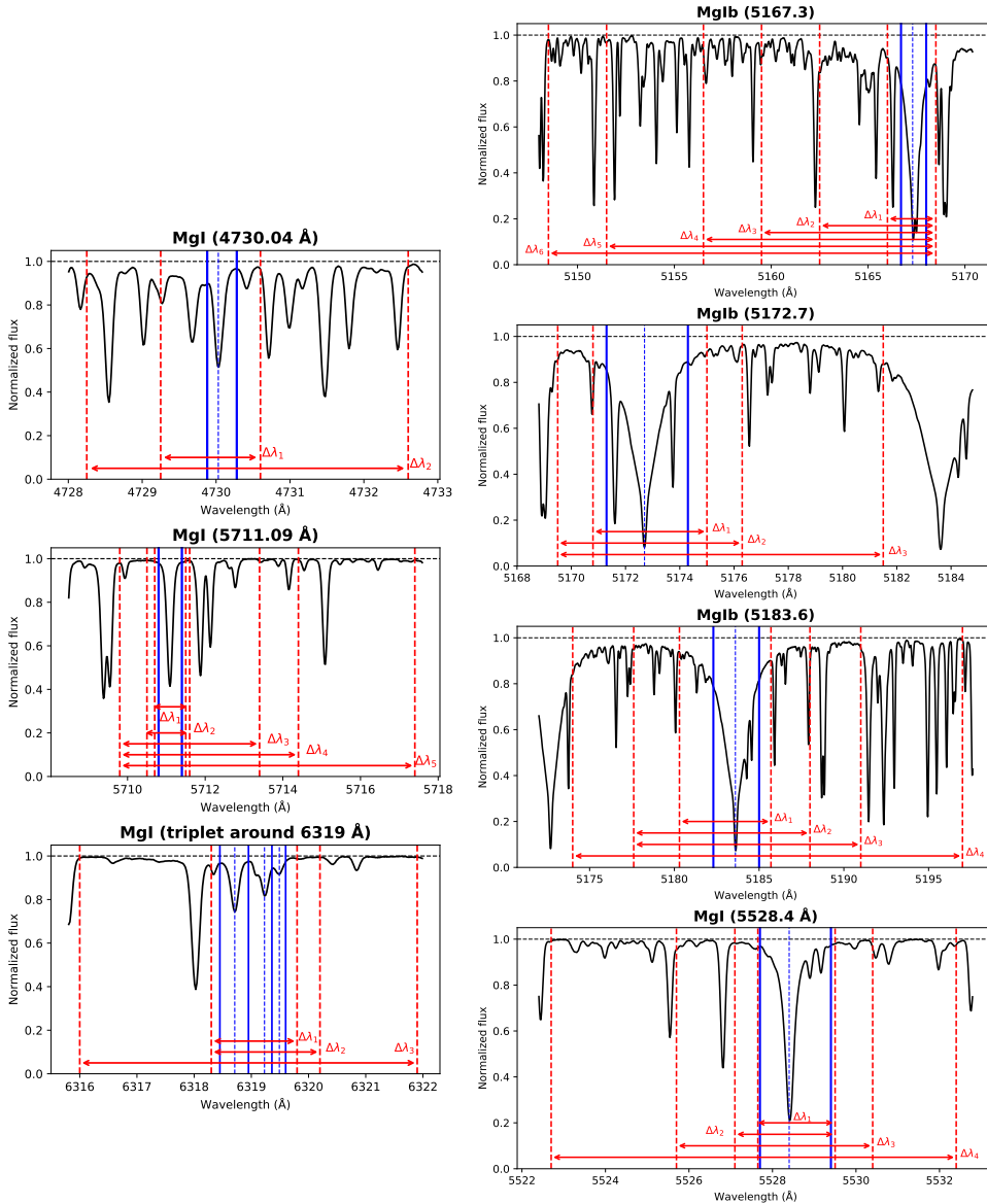
Fig. A.1. Observed solar spectrum from HARPS around each Mg I spectral line. The abundance estimation window is delimited by blue vertical lines ( \Delta\lambda_{\text{Abund}} \sim 0.5 \text{ \AA} for non-saturated lines and \Delta\lambda_{\text{Abund}} \sim 2.5 \text{ \AA} for strong saturated ones). The different local normalisation intervals applied in the analysis are shown with red dashed vertical lines. Left: non-saturated lines: 4730.04, 5711.09, 6318.7, 6319.24, and 6319.49 Å. Right: strong saturated lines: 5167.3, 5172.7, 5183.6, and 5528.4 Å (from top to bottom).
