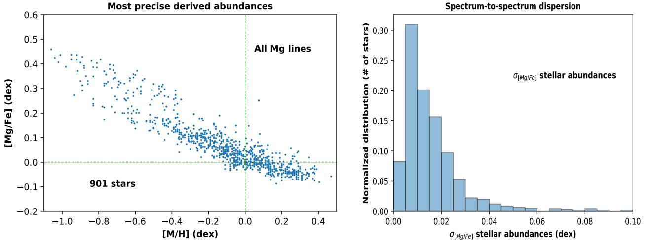
Fig. 17. Left: stellar abundance ratios [\text{Mg}/\text{Fe}] vs. [\text{M}/\text{H}] considering the abundance information from all the studied Mg I spectral lines. Right: estimated dispersion of the final stellar sample ( \geq 4 repeats) on the derived [\text{Mg}/\text{Fe}] abundances.
