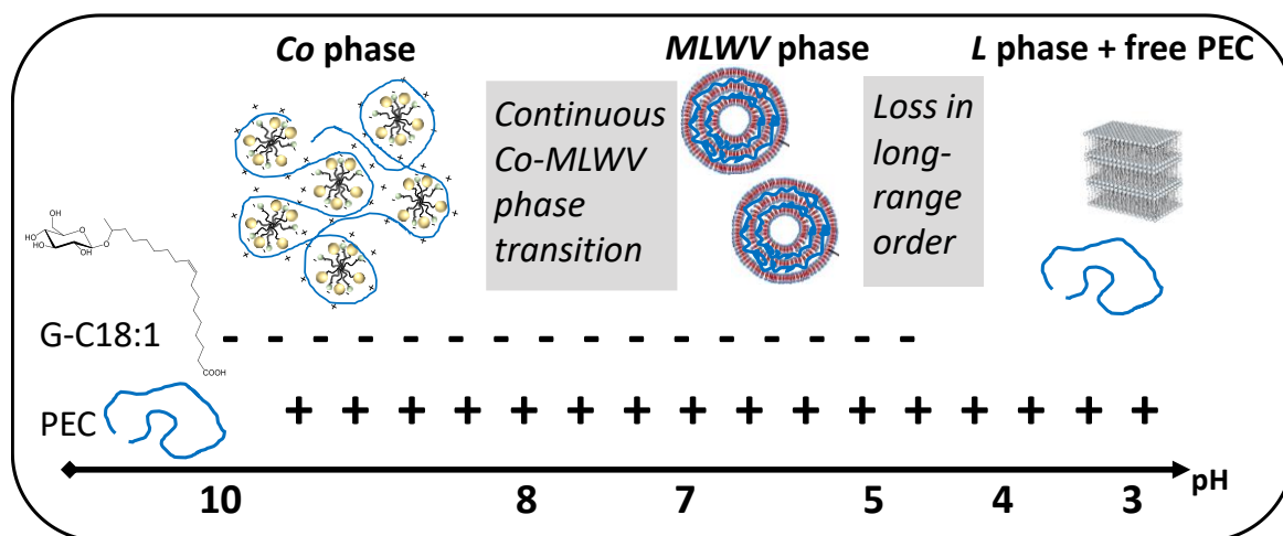
Figure 1 – Phase transition and structures obtained by mixing G-C18:1 and PEC (chitosan, poly-L-lysine, polyallylamine or polyethylenimine) upon a rapid variation of pH. G-C18:1 is negatively charged between about pH 4 and alkaline pH, while PECs are positively charged below pH ~10 (depending on the exact pKa, given in the materials and method section). Complex coacervates ( Co ) composed of G-C18:1 and PEC form
