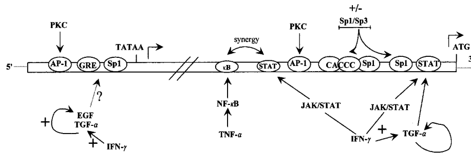
FIG. 11. Schematic representation of the different molecules and signaling pathways involved in MUC4 promoter regulation. Positions of regulatory AP-1, glucocorticoid receptor element, Sp1, CACCC, NF- \kappa B, and STAT binding sites within MUC4 5'-flanking region are indicated. The signals leading to the activation of these transcription factors and that of MUC4 thereafter are shown.
