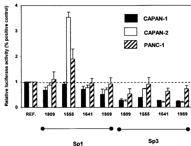
FIG. 7. Transactivating effect of Sp1 and Sp3 on different regions of the promoter of MUC4 . Co-transfection experiments were performed with 1 \mu g of MUC4 deletion mutants (fragments 1809, 1555, 1641, and 1959) and 0.25 \mu g of pCMV4, pCMV-Sp1 or pCMV-Sp3 expression vectors in CAPAN-1 (black bars), CAPAN-2 (white bars), and PANC-1 (hatched bars) cells. The results are the means \pm S.D. and represent more than three different experiments in triplicate for each fragment.
