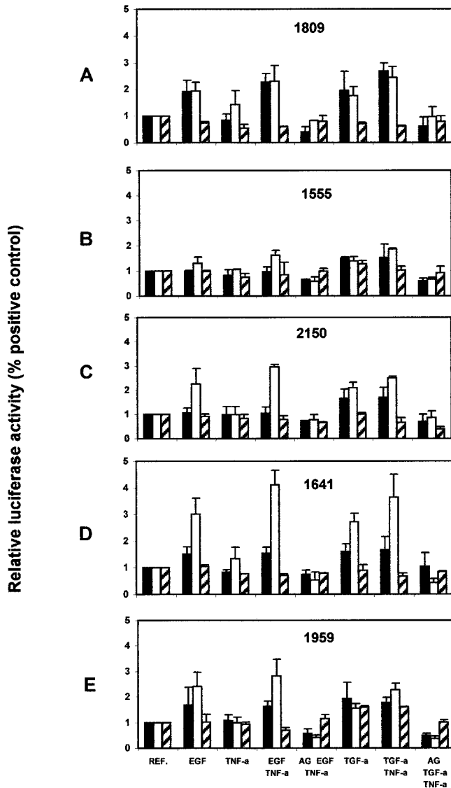
FIG. 9. Effect of EGF, TGF- \alpha , and TNF- \alpha on the activity of MUC4 -pGL3 deletion mutants. Transfected cells (CAPAN-1, black bars; CAPAN-2, white bars; and PANC-1, hatched bars) were treated as described under "Experimental Procedures" before measurement of the luciferase activity of the deletion mutants of interest. REF. refers to the activity of the fragments of interest without any treatment. AG refers to the tyrosine kinase inhibitor tyrphostin AG1478. The results are the means \pm S.D. and represent more than three different experiments in triplicate for each fragment.
