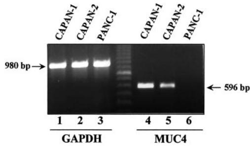
FIG. 3. Expression of MUC4 in pancreatic cancer cells by RT-PCR. RT-PCR on 1.5 \mu g of RNA from CAPAN-1 (lanes 1 and 4), CAPAN-2 (lanes 2 and 5), and PANC-1 (lanes 3 and 6) cells used for cDNA synthesis. Glyceraldehyde-3-phosphate dehydrogenase ( GAPDH , lanes 1–3) and MUC4 (lanes 4–6) PCR products are 980 and 596 bp long, respectively. PCR products were separated on a 1.5% agarose gel run in 1 \times Tris borate-EDTA buffer.
