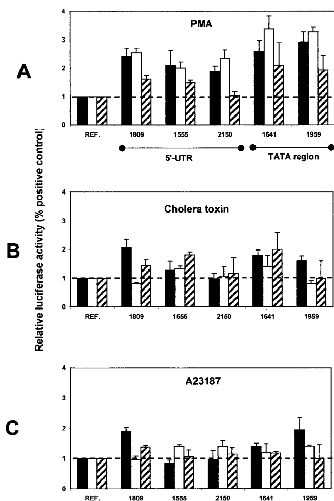
FIG. 8. Effect of PMA, cholera toxin, and A23187 on the activity of MUC4 -pGL3 deletion mutants. Transfected cells (CAPAN-1, black bars; CAPAN-2, white bars; and PANC-1, hatched bars) were treated as described under "Experimental Procedures" before measurement of the luciferase activity of the deletion mutants of interest. REF. refers to the activity of the fragments of interest without any treatment. The results are the means \pm S.D. and represent more than three different experiments in triplicate for each fragment.
