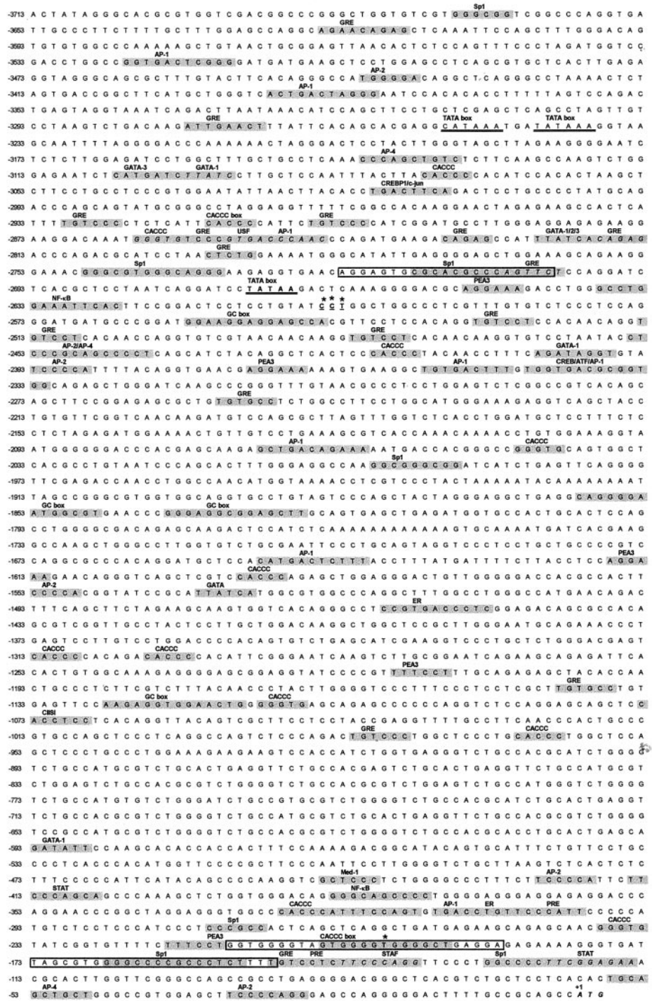
FIG. 2. Sequence of the promoter region and 5'-UTR of the human mucin gene MUC4. The three putative TATA boxes are double-underlined, and putative binding sites for known transcription factors are in gray. The transcription start sites at -199, -2603, -2604, and -2605 are in bold type and marked with an asterisk. The sequences of the oligonucleotides used for EMSA studies are boxed. The first ATG is in bold type and italicized. Numbering refers to the first ATG designated +1.
