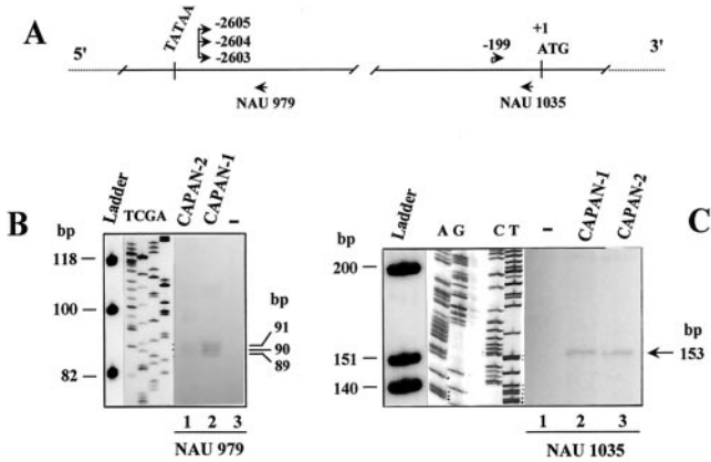
FIG. 4. Identification of multiple transcription start sites within the 5'-flanking region of MUC4 using primer extension. A, positions of the transcription start sites are indicated on the schematic view of the 5'-flanking region of MUC4 and numbering refers to the translational start site of MUC4 . The positions of the reverse primers used in primer extension experiments are indicated. B, primer extension on 20 \mu g of total RNA from CAPAN-2 (lane 1) and CAPAN-1 (lane 2) cells. Lane 3, no RNA added. Three extension products of 89, 90, and 91 bp (lanes 1 and 2) were produced when using NAU 979 reverse primer located downstream of the TATA box. C, primer extension on 20 \mu g of total RNA from CAPAN-1 (lane 2) and CAPAN-2 (lane 3) cells. Lane 1, no RNA added. One extension product of 153 bp was produced (lanes 2 and 3) when using NAU 1035 reverse primer located in the 3'-end of the 5'-UTR. \phi X174 DNA/ Hinf I dephosphorylated markers previously radiolabeled and denatured are indicated on the left side of the gels. The sequence of the M13mp18 plasmid control is shown.
