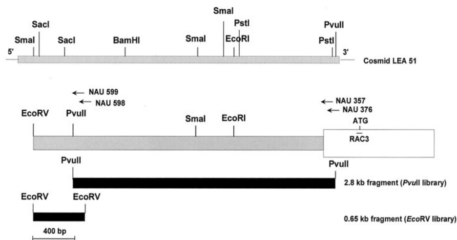
FIG. 1. Schematic representation of the genomic clones covering the 5'-flanking region of human mucin gene MUC4 upstream of the ATG. The 3'-end of the cosmid LEA 51 is shown and aligned with the PvuII 2.8-kb clone and the EcoRV 0.65-kb clone obtained with the Genome walker kit.
