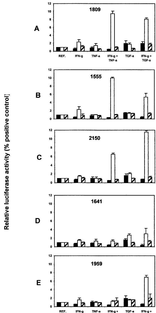
FIG. 10. Study of the synergistic effect of IFN- \gamma , TNF- \alpha and TGF- \alpha . Transfected cells (CAPAN-1, black bars; CAPAN-2, white bars; and PANC-1, hatched bars) were treated as described under "Experimental Procedures" before measurement of the luciferase activity of the deletion mutants of interest. REF. refers to the activity of the fragments of interest without any treatment. The results are the means \pm S.D. and represent more than three different experiments in triplicate for each fragment.
