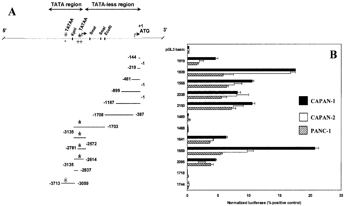
FIG. 5. Position and transcriptional activity of MUC4 pGL3 deletion mutants in pancreatic cancer cell lines. A , schematic representation of the localization of the different pGL3 deletion mutants covering 3721 nucleotides upstream of the first ATG. The numbering refers to the translational start site designated +1. The TATA box locations are indicated as well as some restriction sites found in the 5'-flanking region of the gene. B , transcriptional activity of the deletion mutants was studied in CAPAN-1 (black bars), CAPAN-2 (white bars), and PANC-1 (hatched bars) cell lines. The background activity of pGL3 Basic promoterless vector used to subclone MUC4 fragments is shown. The results are the means \pm S.D. and represent more than three different experiments in triplicate for each fragment.
