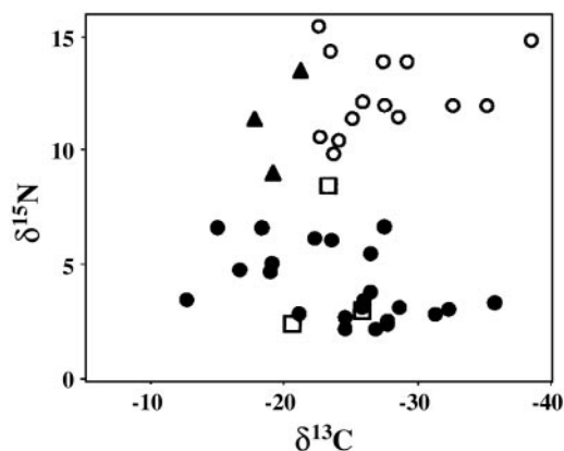
Fig. 2. Paired \delta^{13}\text{C}/\delta^{15}\text{N} values (‰) for OM. ●, symbiotic; ○, nonsymbiotic; ▲, Oculina spp.; □ P. major .
