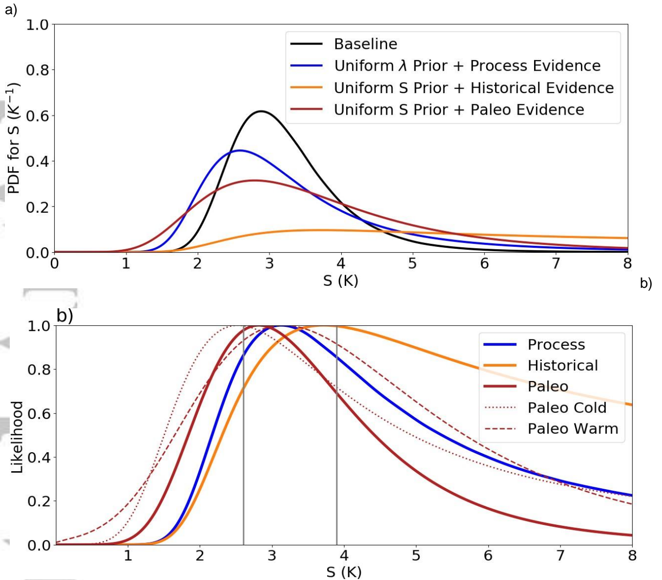
Figure 20 . Posterior PDF for S and comparison of lines of evidence. Panel (a) shows our Baseline posterior PDF for S in black, and PDFs for each main line of evidence individually, where the process evidence is combined with a uniform \lambda prior while the others are combined with a uniform prior on S . (b) shows marginal likelihoods for S for the various lines of evidence used in the Baseline calculation: the individual-feedback process evidence (section 3); the likelihood from historical evidence (section 4); and the likelihoods for past warm and cold climates from paleoclimate evidence plus their combined likelihood (section 5). All likelihoods are scaled to have a maximum value of unity. Vertical grey lines show the 66% range for the Baseline posterior for S .
