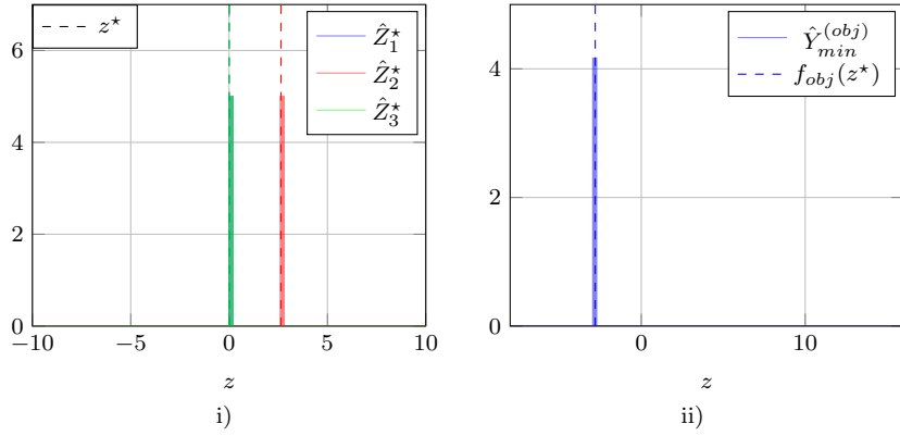
Fig. 21 Application example. i) Histograms of the minimum value position \hat{Z}^* ii) Histogram of the minimum value \hat{Y}_{min}^{(obj)} after 10 iterations of Algo. 2.
