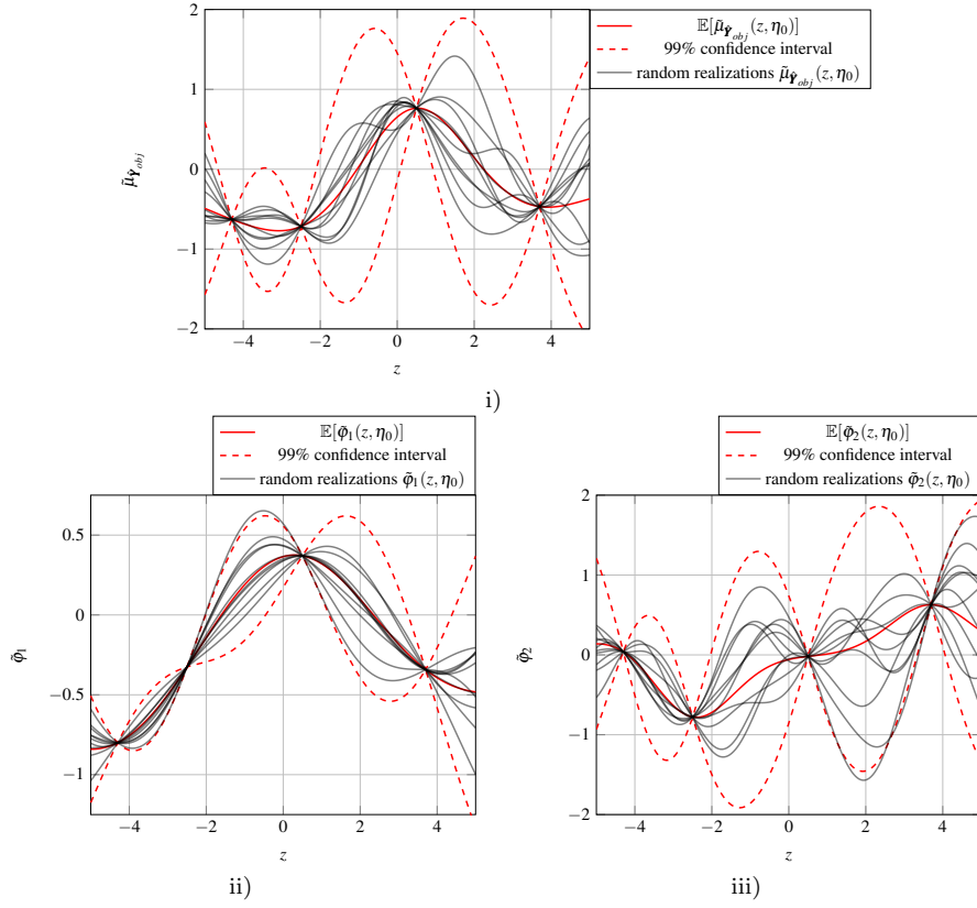
Fig. 7 1-D toy problem. Illustration of the GP interpolation used in Eq. (14). Mean GP approximation (red solid line), 99% confidence interval (dashed red lines), random realizations (black solid lines) i) Mean value of the KL decomposition ii) First eigenvector of the KL decomposition iii) Second eigenvector of the KL decomposition.
