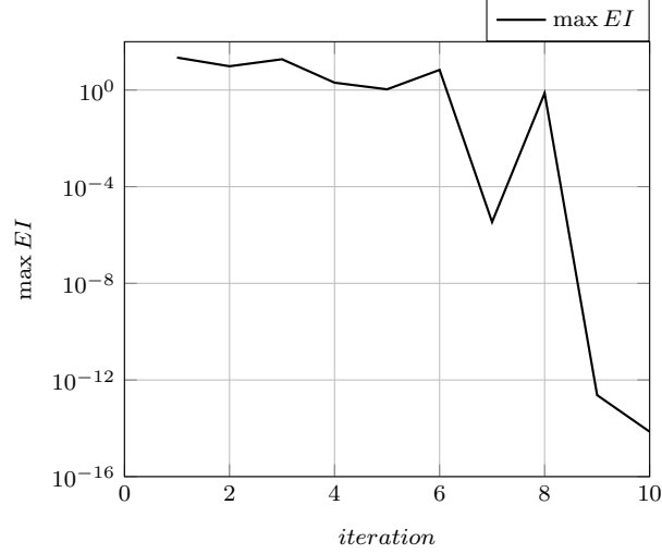
Fig. 20 Application example. Evolution of the maximum value of the EI defined by Eq. (16) with respect to the number of iterations of the proposed EGMDO algorithm.
