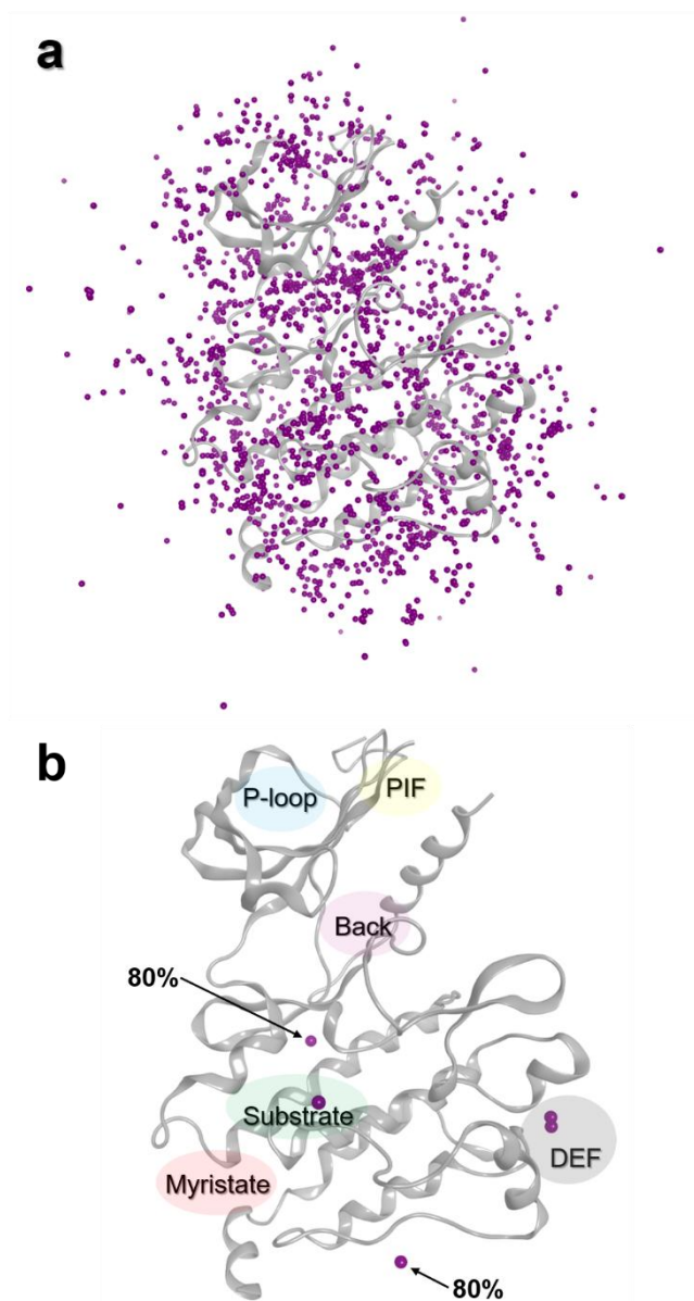
Figure 2. Distribution of CA centroids around a PK (PDB ID 1K5V). (a) Representation of all CA centroids. (b) Position of centroids with density greater than 80% (centroids indicated by an arrow) and 50% (all purple spheres).
