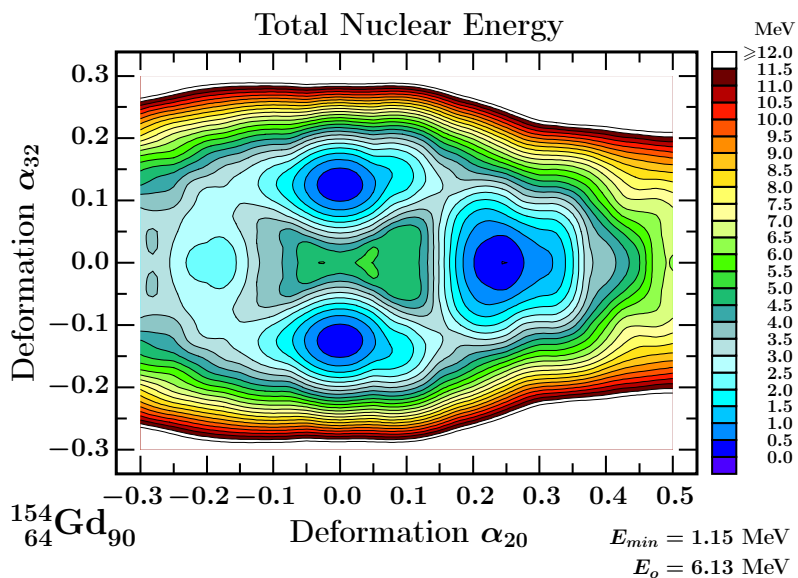
Fig. 1. Shape competition: Quadrupole minimum at \alpha_{20} \approx 0.22 , and tetrahedral one with symmetric minima at \alpha_{32} \approx \pm 0.12 ; Woods-Saxon mean-field, Ref. [7].
