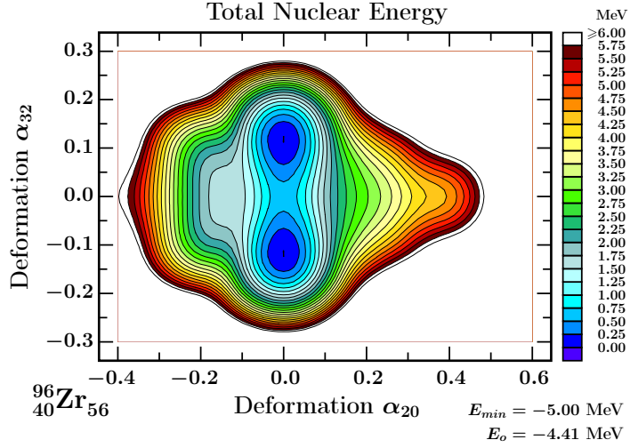
Fig. 5. Total nuclear energy surface for ^{96}\text{Zr} projected onto the (\alpha_{20}, \alpha_{32}) deformation plane showing two symmetric tetrahedral symmetry minima at \alpha_{32} \approx \pm 0.12 . The importance of this indication is enforced by the results presented in Table 1 and showing a very high value of the B(E3) value associated with the first I^\pi = 3^- excitation in this nucleus.
