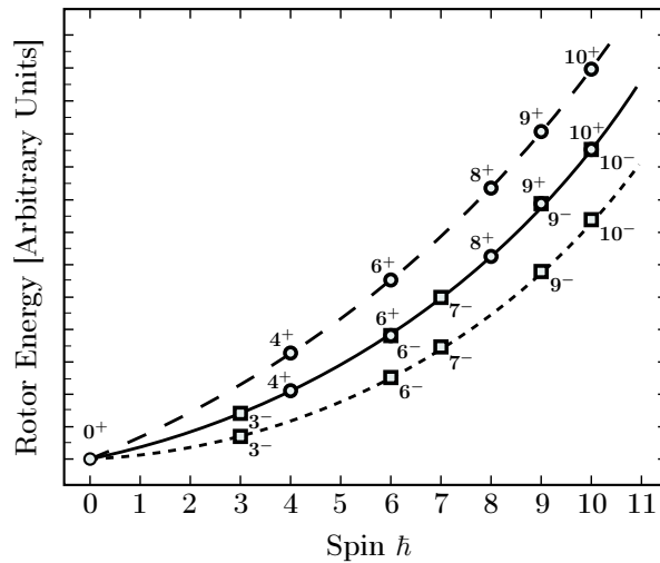
Fig. 3. Schematic: Tetrahedral symmetry band, full line, composed simultaneously of positive and negative parity states, some of them ( 6^\pm , 9^\pm , 10^\pm ) degenerate, cf. Eq. (1). Dashed lines illustrate the positive and negative parity octahedral band-partners, cf. Eqs. (2-3). According to the discussed criteria, the pure tetrahedral symmetry case should result in one band with both parity states forming approximately a common parabola whereas dominating octahedral symmetry might lead to two close-lying but well separated bands of opposite parities as schematically illustrated.
