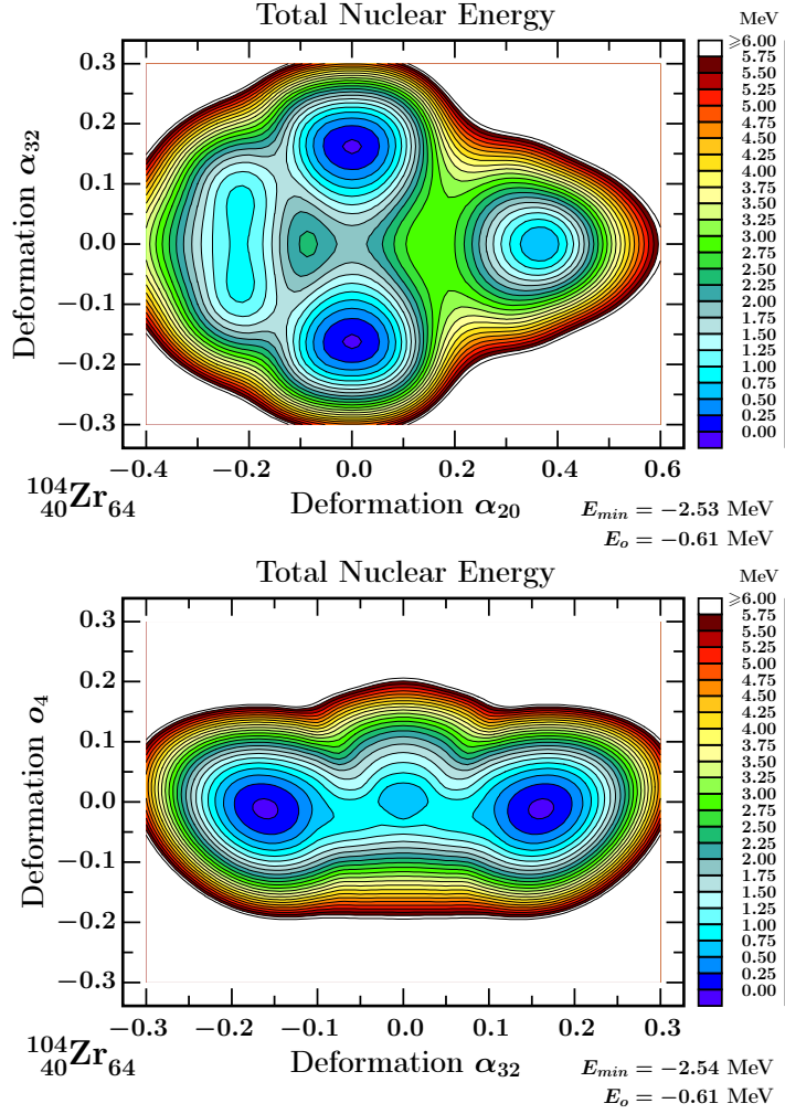
Fig. 7. Top: Total nuclear energy surface for ^{104}\text{Zr} projected onto the (\alpha_{32}, \alpha_{20}) deformation plane. Bottom: total nuclear energy projected onto the (\alpha_4, \alpha_{32}) deformation plane. In this case the pure tetrahedral deformed minimum appears to be again the ground state but the strongly deformed ( \alpha_{20} \sim 0.38 ) and oblate ( \alpha_{20} \sim -0.2 ) shapes are also predicted.
