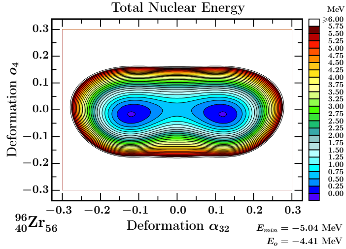
Fig. 6. Illustration similar to the one in Fig. 4 showing two symmetric tetrahedral symmetry minima at o_4 \approx 0 indicating no coexistence between tetrahedral and octahedral degrees of freedom in contrast to the previous case; these results predict a pure tetrahedral symmetry configuration.
