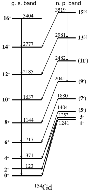
Fig. 2. Experimental results for the two rotational bands in ^{154}\text{Gd} ; the data are from Ref. [8].
