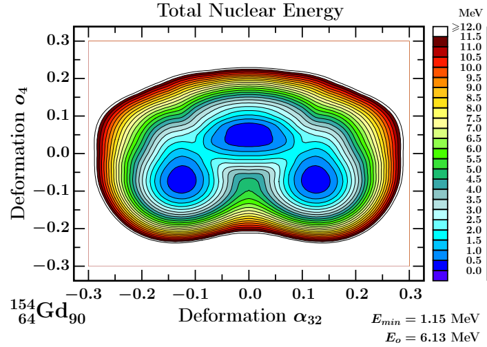
Fig. 4. Total energy calculations analogous to those shown in Fig. 1 but for the octahedral ( o_4 \leftrightarrow \{\alpha_{40}, \pm\sqrt{5/14}\alpha_{4,\pm 4}\} ) and tetrahedral ( \alpha_{32} ) deformation projection; for the exact definition of the octahedral deformation cf. Ref. [13]. These results suggest two high-rank symmetry mechanisms: Pure octahedral symmetry configuration corresponding to \alpha_{32} \approx 0 at o_4 \approx 0.06 , and the double minimum of the combined tetrahedral, \alpha_{32} \approx \pm 0.13 , and octahedral, o_4 \approx -0.08 deformations.
