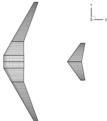
Figure 6: VLM model of the CeRAS baseline - top view.
