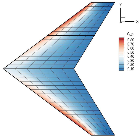
Figure 2: Warren-12 wing VLM model decomposed in four wings to validate the interaction of multi-wing configurations.
