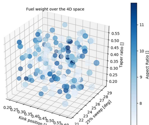
Figure 11: 5D visualization of fuel weight predictions. The size of the spheres is proportional to the normalized fuel weight. Results obtained with L1 aerodynamic model.
