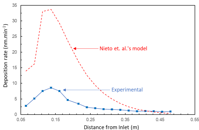
Fig. 4. Average calculated deposition rates of run E3 (SP 400°C), simulated using Nieto et al.'s model (red dashed line) and compared to the respective experimental average deposition rates per coupon (blue squares).
