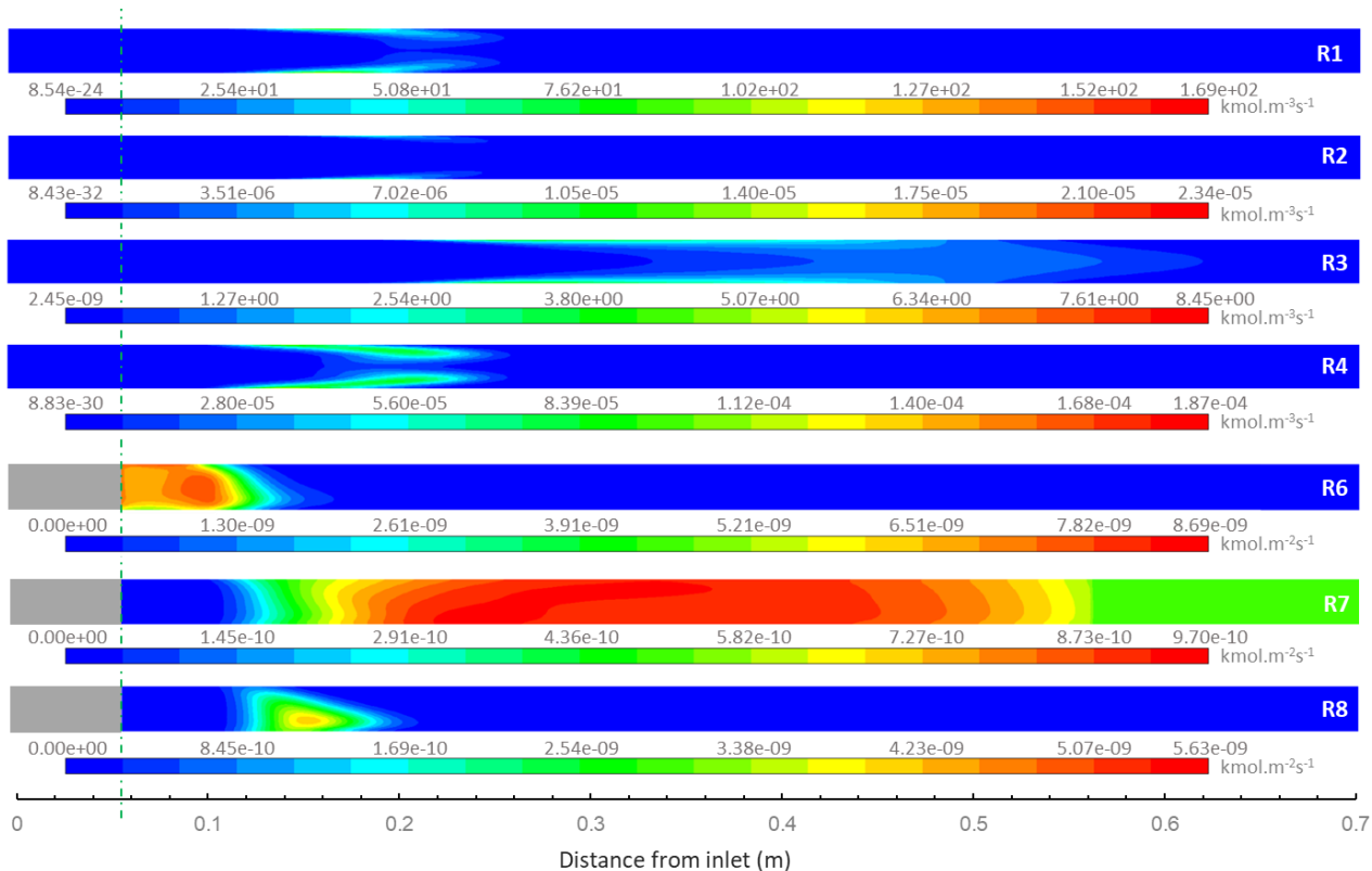
Fig. 10. Reaction rate profiles for all reactions plotted along the XZ plane for the gas phase reactions ((R1) to (R4)) and along the YZ plane for the surface reactions ((R6) to (R8)) of run E4 (450°C). Vertical green dash-dotted line signifies the start of the substrates.
