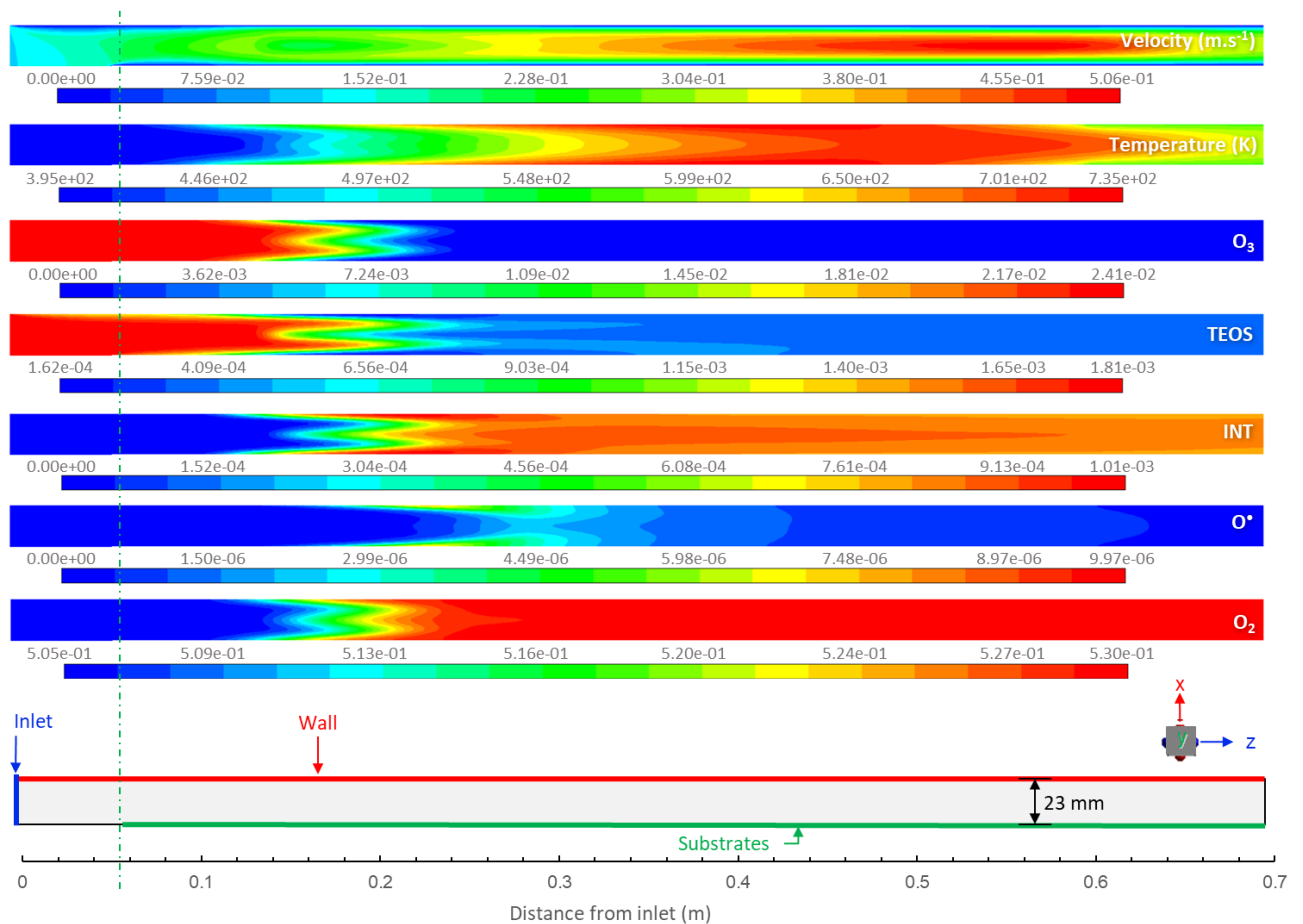
Fig. 9. Local velocity, temperature and mass fraction profiles of TEOS, INT, O 3 , O 2 and O* plotted along the XZ plane for run E4 (450°C). Vertical green dash-dotted line signifies the start of the substrates at 0.057 m.
