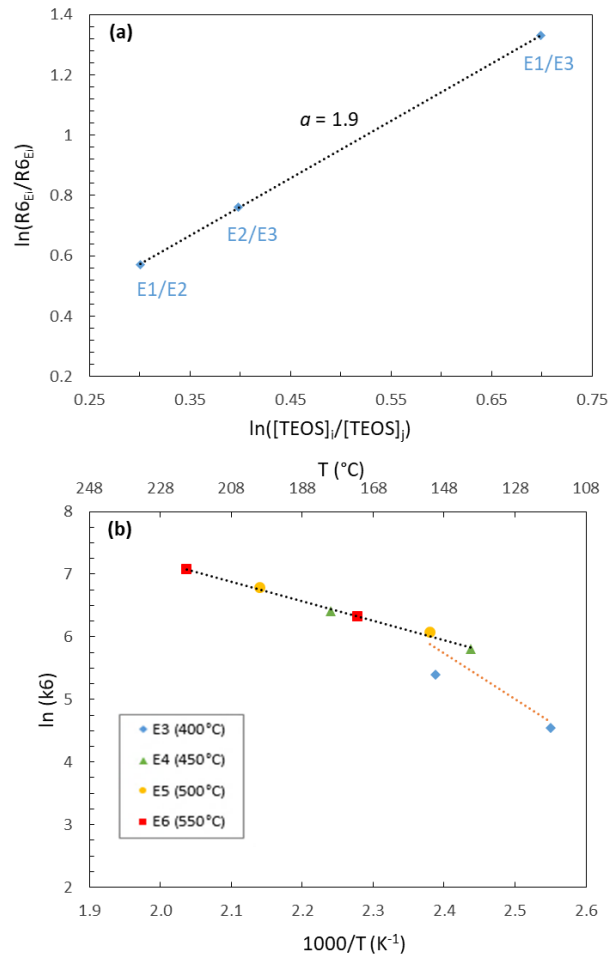
Fig. 5. (a) Determination of partial order exponent for TEOS in reaction (R6). (b) Linear interpolation of k_6 logarithm versus the inverse temperature, plotted for selected samples of runs E3 to E6.
