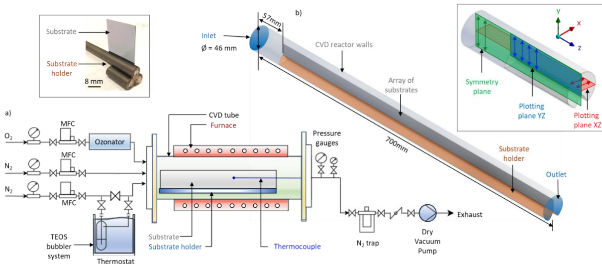
Fig. 1. Schematic (a) and 3D (b) representation of the CVD reactor (not true-to-size and proportion). Top left inset photograph shows the substrate holder supporting a Si coupon vertically. Top right inset scheme depicts the symmetry plane, the plotting plane YZ used for surface results presentation and the plotting plane XZ used to present gas phase results.
