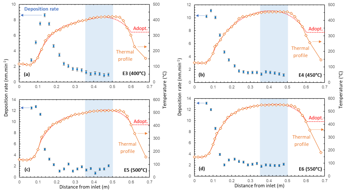
Fig. 3. Evolution of the experimental deposition rates (blue circles), the reactor's thermal profile (orange diamonds), and the adopted thermal profile (red dashed line), along the reactor length, for runs E3 (a), E4 (b), E5 (c) and E6 (d). Light-blue rectangles depict the considered isothermal regions.
