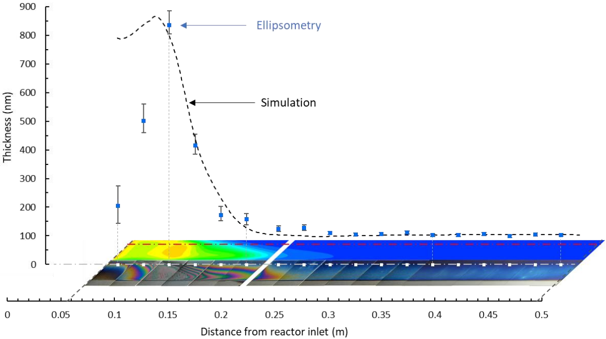
Fig. 8. Comparison of calculated local thickness (dashed black line) from simulations, and experimental local thickness (blue squares) measured by a refractive ellipsometer for run E4. Photograph of array of samples and scale denoting distance from the reactor inlet are included for visual aid. Red dashed-dotted line represents the line along which the simulation results were extracted. White squares represent the points at which the ellipsometric measurements were taken.
