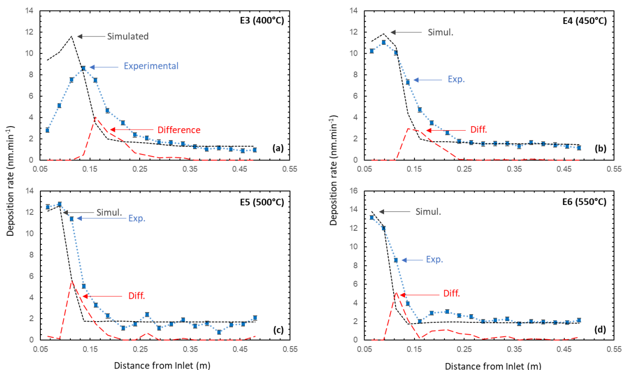
Fig. 6. Evolution of average experimental deposition rate on each sample (blue squares), average simulated total deposition rate (black dashed line) calculated for each sample, after simulating reactions (R1) to (R7) of the model. Difference of average experimental minus average simulated total deposition rate, for the samples on which the simulation underestimates the experimental rate (red dashed line). (a) Run E3, (b) E4, (c) E5, and (d) E6.
