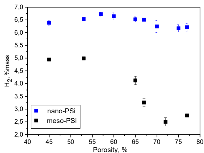
Figure 9. Porosity dependent hydrogen generation amount due to oxidation reaction of meso- and nano-PSi powders in H 2 O:Ethanol:NaOH solutions at room temperature. Alkali concentration was 0.5 M/L.
