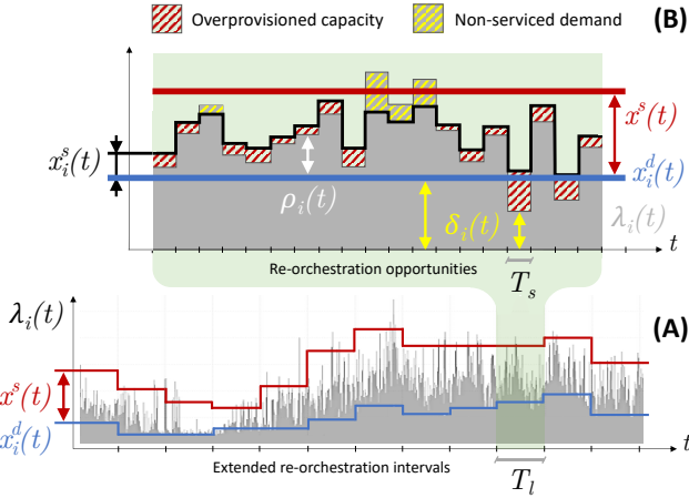
Fig. 2. Orchestration model. (A) Long-timescale orchestration. The background time series represents the traffic demand generated by slice i (grey). The curves portray the time evolution of the dedicated capacity x_i^d(t) allocated to slice i (blue), and of the shared capacity x^s(t) (red) over extended intervals of duration T_l . Note that x^s(t) is added to the dedicated resources to determine the total available capacity, and, unlike x_i^d(t) , is not reserved for slice i but available to all slices. (B) Short-timescale orchestration during one extended interval. At every T_s < T_l , a portion x_i^s(t) (black solid curve) of the (fixed) shared capacity x^s(t) is allocated to slice i , based on the residual demand \rho_i(t) not satisfied by the (fixed) dedicated resources x_i^d(t) . The plot also highlights the volume of overprovisioned capacity and non-served demand (pattern regions), and the slice traffic below dedicated capacity \delta_i(t) .
