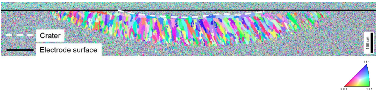
Fig. 8. Inverse pole figure map for silver obtained in the normal direction to the sample cross-section of an anode cross section along a crater diameter after a single arc (300 A rms current).
