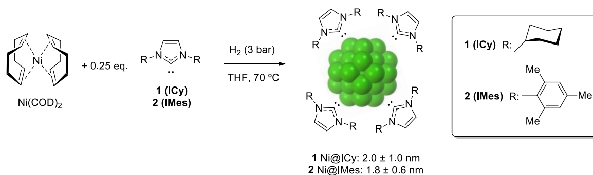
Scheme 1 Synthesis of Ni@NHC NPs 1 and 2 .
