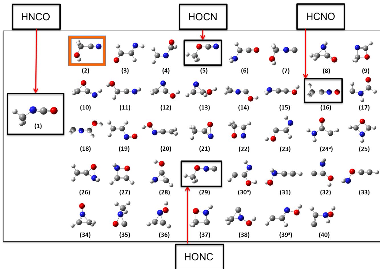
Fig. 1. Structures of C_2H_3NO isomers as ordered in Table 1 by increasing energy. The black boxes correspond to the HNCO isomers (Table 2), the orange box corresponds to the second isomer HOCH_2CN identified recently. (a) Isomer whose electronic ground state is a triplet state.
