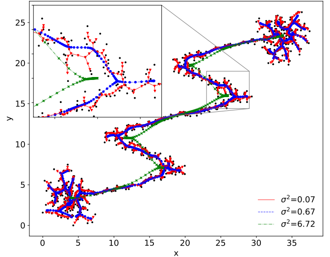
Fig. 8. Effect of the \sigma parameter on the regularised MST by fixing \lambda = 1 . Black dots are data points while red, blue and green lines are RMST with respectively \sigma^2 = \{\frac{\sigma_s^2}{10}, \sigma_s^2, 10\sigma_s^2\} (see Eq. (14)). Corresponding projected points are also represented, respectively, by triangles, dots and crosses.
