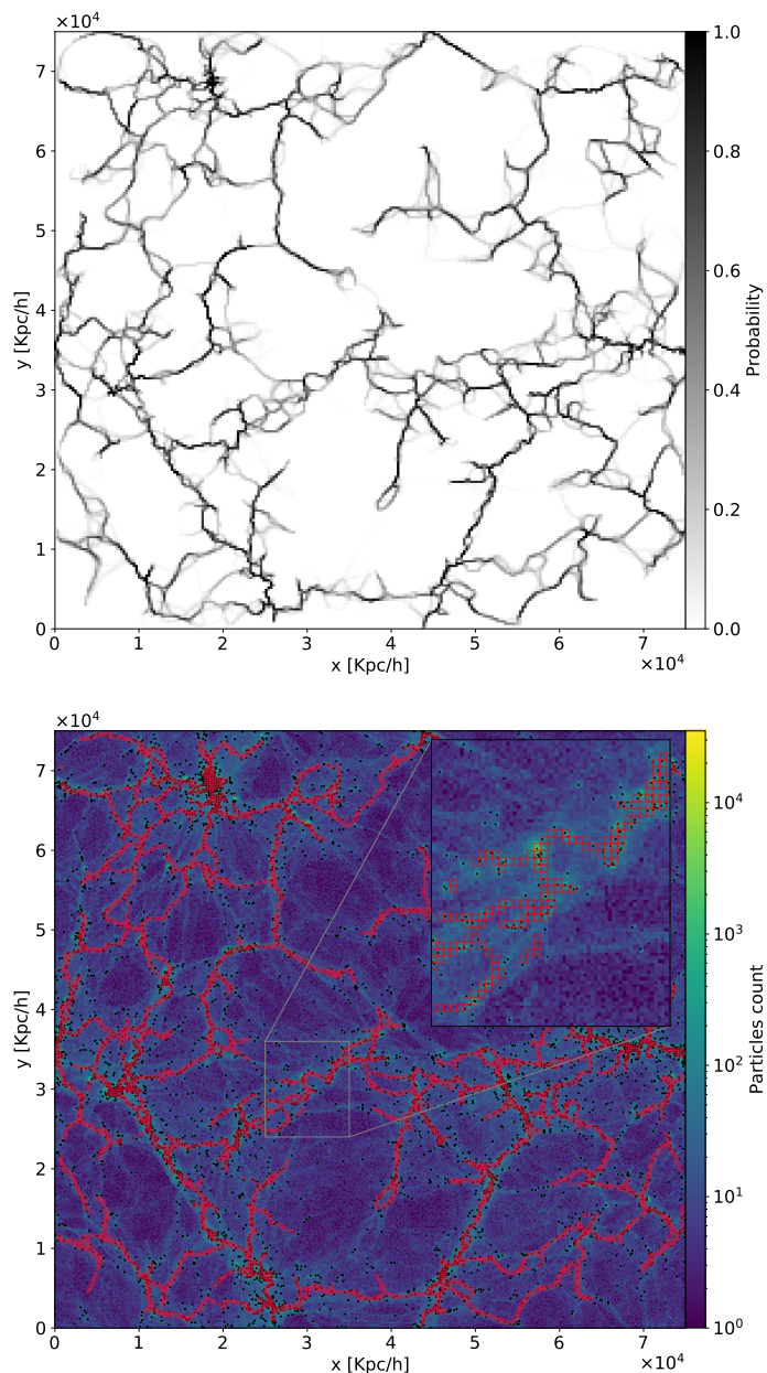
Fig. 12. Top: probability map \mathbf{I} obtained from subhalos displayed in Fig. 2 with parameters described in Table 1. The resolution of the probability map is 250 \text{ Kpc h}^{-1} . Bottom: superlevel set \Gamma_{0.25}(\mathbf{I}) (red squares) overlapped on the DM distribution together with subhalos (black dots).
