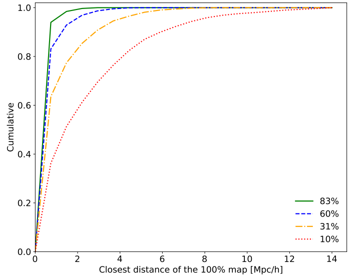
Fig. 15. Cumulative distribution of distances \{d_x^J\} (see Sect. 6.1.2) obtained with increasing mass threshold M^{\text{cut}} to the one with J\% of the data points. M^{\text{cut}} = \{0.85, 1.35, 3.22, 11\} \times 10^{10} M_{\odot} h^{-1} leading respectively to 83%, 60%, 31% and 10% of the total number of subhalos in the slice.
