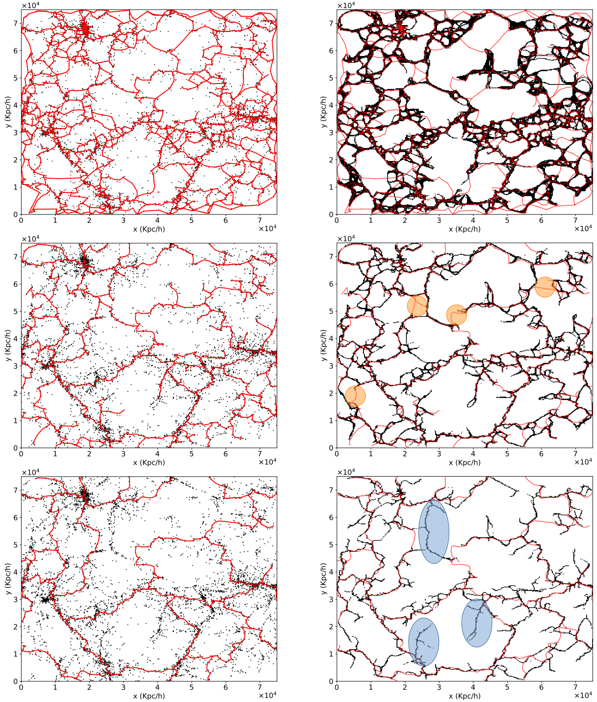
Fig. 13. Left column: subhalos (black dots) and DisPerSE skeletons (red lines) with several significance levels ( from top to bottom: \sigma_p = 0, 2, 5 ). Right column: superimposition of some thresholded probability maps obtained by T-ReX and DisPerSE skeletons (red lines) with several significance levels ( from top to bottom: \sigma_p = 0 and \Gamma_{0,0}(\mathbf{I}) , \sigma_p = 2 and \Gamma_{0,1}(\mathbf{I}) , \sigma_p = 5 and \Gamma_{0,25}(\mathbf{I}) ). Resolution of the maps provided by T-ReX is 250 \text{ Kpc h}^{-1} . Shaded blue and orange areas highlight some differences between results discussed in Sect. 6.1.1.
