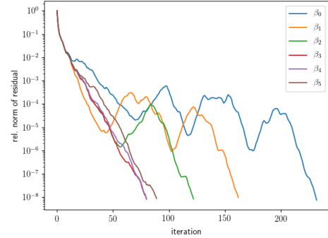
Fig. 4. Convergence of deflated PCG with the deflation subspace built by recycling. Here we consider the first six systems from the sequence and start the iterations always with zero initial guess. k = 10 eigenvectors are approximated using \text{dim}_p = 100 .
