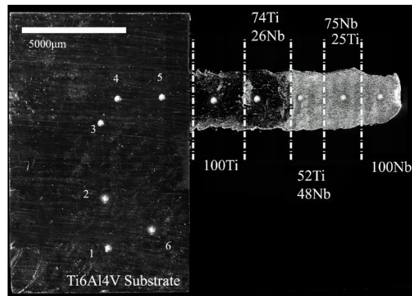
Figure 3: Chemical composition of each zone of the Ti-Nb wall, and position of indentation in the wall and in the substrate realized in face 1 of the Ti-Nb part
