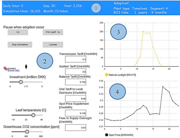
Fig. 4. The interface of a running simulation in AnyLogic.
