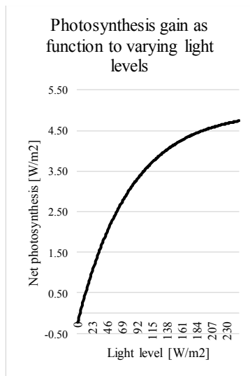
Fig. 5. Photosynthesis function to the light level with constant CO 2 level and leaf temperature.
