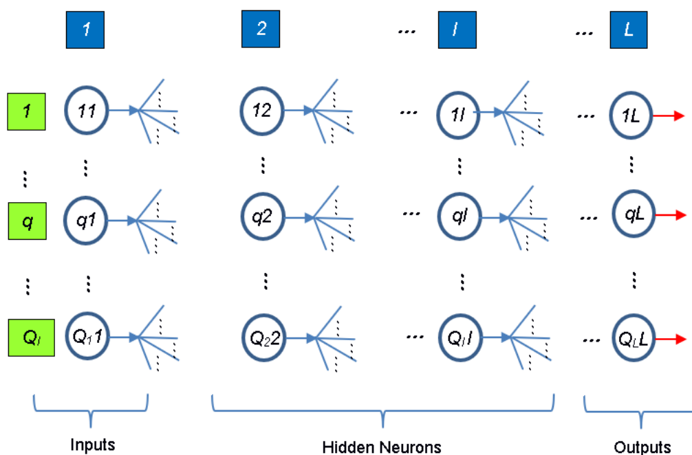
Fig. 4. Generic multi-layer feedforward network.
