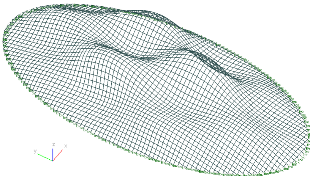
Fig. 1.1. 1 st buckling mode of a paraboloid shell (model 1030) supported along its perimeter.
