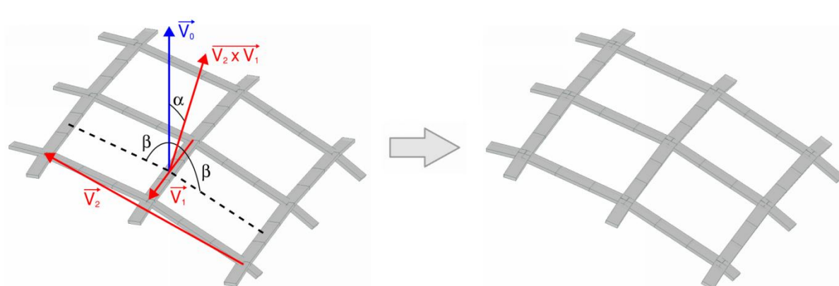
Fig. 1.3. Procedure carried out to rotate each beam's coordinate system in all grid-shells.
