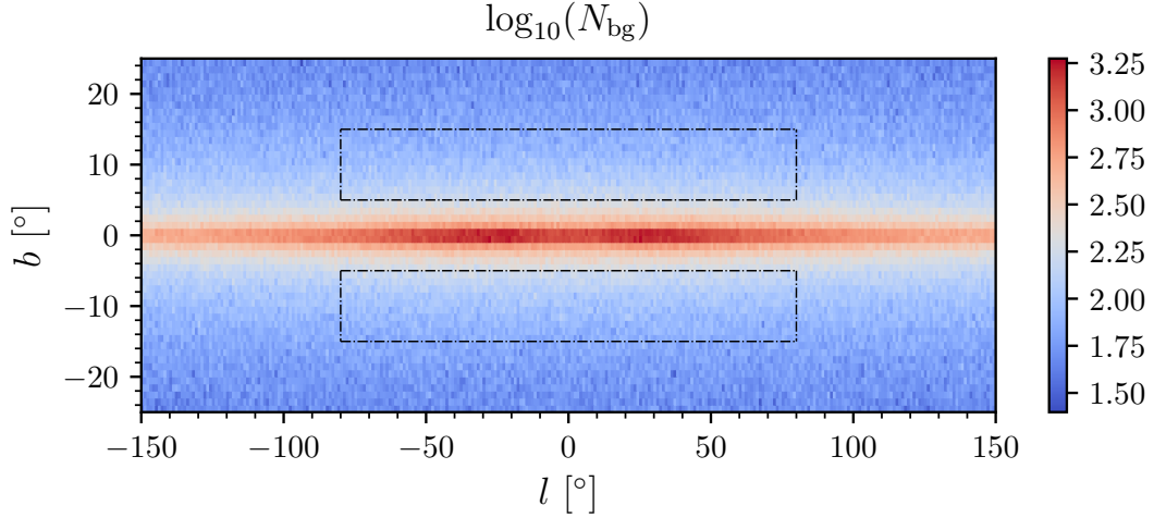
FIG. 9. Mock photon count map of biased background photons received in bins of size 1^\circ \times 1^\circ in the range 1-100 GeV. We used bias parameters \hat{\alpha}_b = 1.3 and \eta = 0 . The contour areas correspond to the RoI used to set constraints on \langle\sigma v\rangle .
