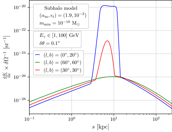
FIG. 14. Distance distribution of the visible subhalos. The background is J_\infty with the replacement \delta\Omega = \delta\Omega = 2\pi(1 - \cos(\delta\theta)) and n_\sigma/\tilde{n}_\sigma = 2 - the parameters of the subhalo model are the same than in Fig. 7. The energy range is 1 \text{ GeV} < E_\gamma < 100 \text{ GeV} . Note that since we treated the opening angle as a free parameter this map is independent of the DM mass (provided it is above 1 GeV) and of its annihilation channel.
