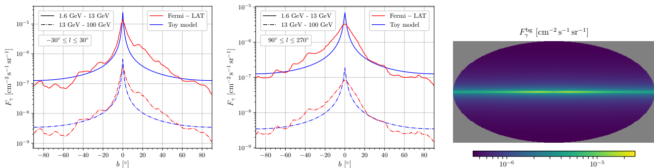
FIG. 4. Left panel: Latitudinal profiles calculated from the flux given Eq. (46) and integrated in two energy ranges, [1.6-13] GeV (top plain curves) and [13-100] GeV (bottom dot-dashed curves), and averaged in the longitudinal range -30^\circ \leq l \leq 30^\circ . The model (blue curves) is compared with the Fermi data (red curves). Middle panel: Same as in the left panel, but averaged in the longitudinal range 90^\circ \leq l \leq 270^\circ . Right panel: Full skymap the the background flux integrated in the [1.6-13] GeV energy range, which also contains the isotropic component—see Eq. (48).
