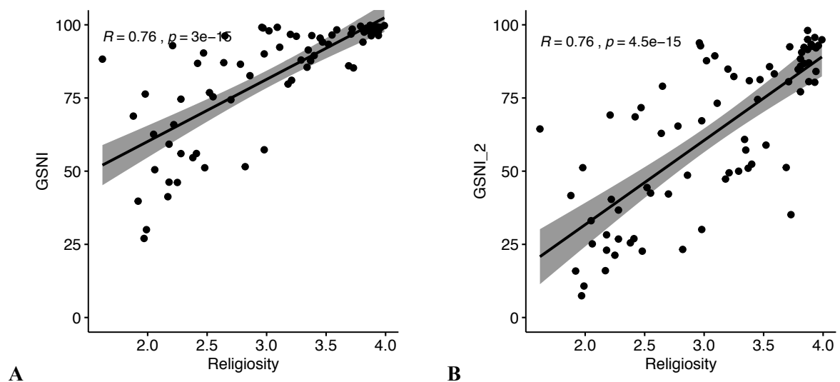
Figure 2 – Pearson correlations between Religiosity and (A) GSNI ( N = 75 countries, R = 0.76, p < 0.001 ), (B) GSNI2 ( N = 75 countries, R = 0.76, p < 0.001 ). Grey surfaces: confidence intervals (95%).
