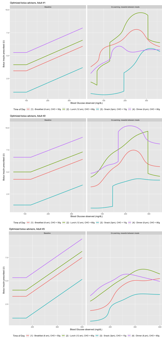
Figure 2: Bolus advisor \pi_0 (left) and \pi_{\bar{\alpha}^*} found by Q-Learning with function approximation (right) for each virtual patient (sorted by increasing number). One can observe essentially two things from those graphs : first, it looks as if patient #1 and #2 are closer to each other than to patient #3 in terms of physiology otherwise we would not find the result we did. However the hope to get out a new generic rule seems difficult in this situation. Second, and this is what shows the algorithm took into account sequentiality of the meals and injections : the meal with most carbs does not necessarily require most insulin, which is a fundamental difference from the baseline advisor.
