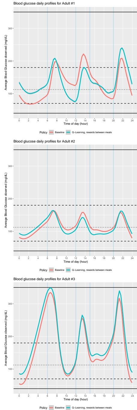
Figure 3: Average BG profiles for the three virtual patients (sorted increasingly by number) for each policy applied, \pi_0 in red and \pi_{\bar{\alpha}^*} in light blue. For all adults, the algorithm basically learned to reduce insulin intake at last meal in order to reduce nightly hypoglycemia at the cost of often minor hyperglycemia. The changes are minor in the case of Adult #2, but in Adult #3 and #1 it centers the BG levels around target 112.5 mg/dL.
