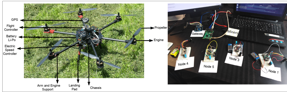
Figure 4: Experiment testbed: a) Hexacopter Drone; b) Blockchain-based platform
