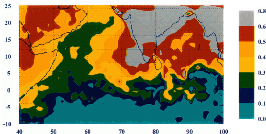
Plate 18. The 3-month (and diurnal) mean heating rate averaged between the surface and 3 km, due to anthropogenic aerosols. The ocean values were obtained from the integrated observations, while the land values were obtained from the 4-D assimilation model of Collins et al. [2001].
